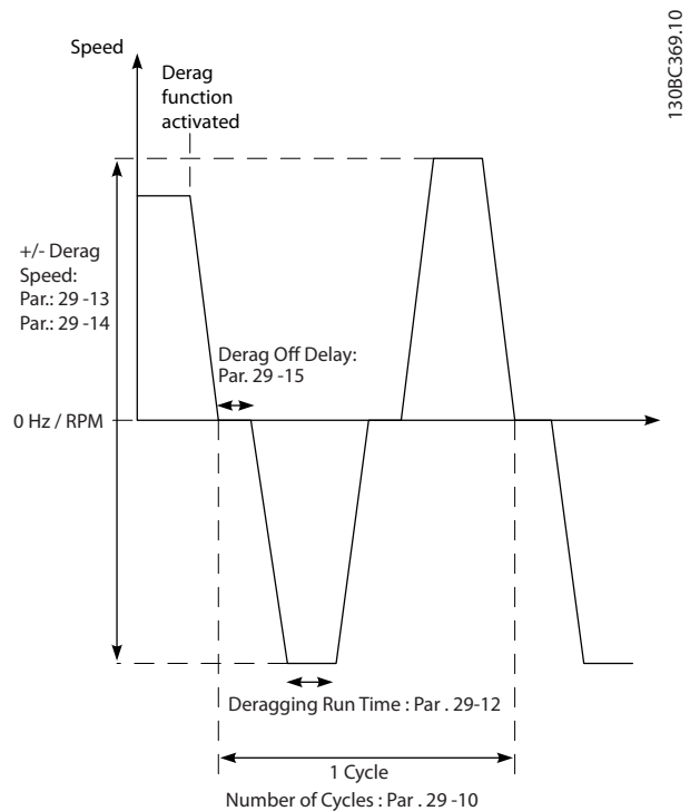
Illustration 5.12 Derag Function
