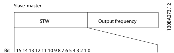
Illustration 14.17 STW Slave-to-Master
