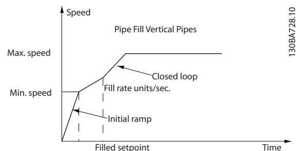
Illustration 12.6 Performance Curve for Pipe Fill Mode
