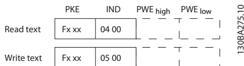
Illustration 14.11 PWE
