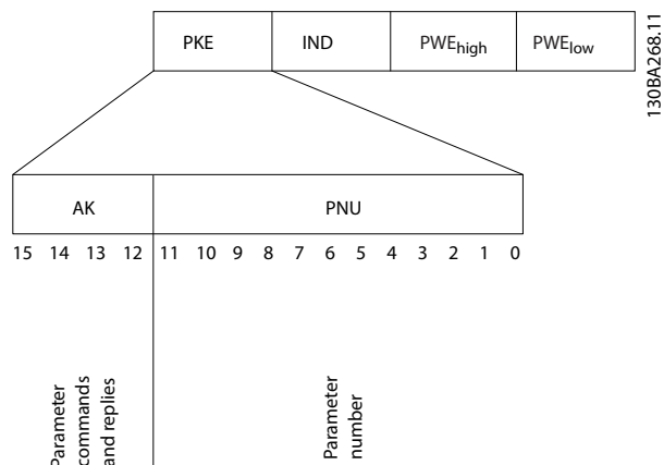
Figure 14.10 PKE Field
