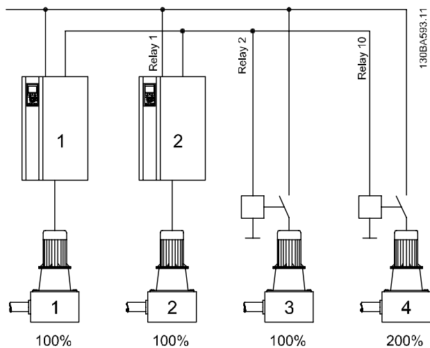
Figure 5.10 Basic Cascade Controller
