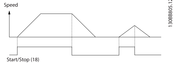
Figure 12.1 Start/Stop with Safe Torque Off
