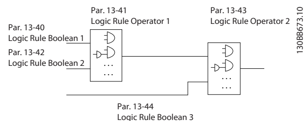
Figure 5.6 Logic Rules
