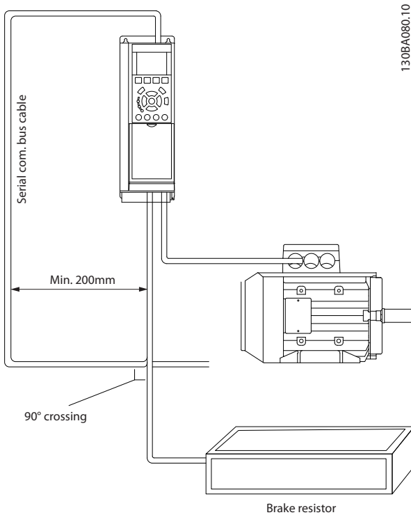
Figure 14.4 EMC Precautions
