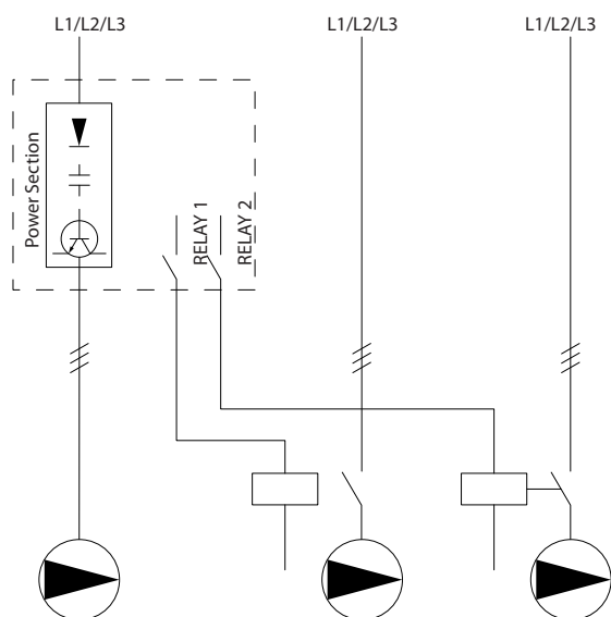
Figure 12.7 Fixed Variable Speed Pump Wiring Diagram
