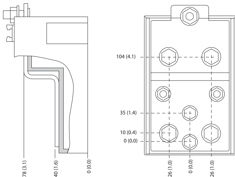
Figure 8.3 Detailed Terminal Dimensions for E1/E2
