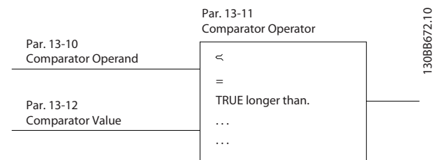
Figure 5.5 Comparators
