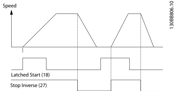
Figure 12.2 Latched Start/Stop Inverse
