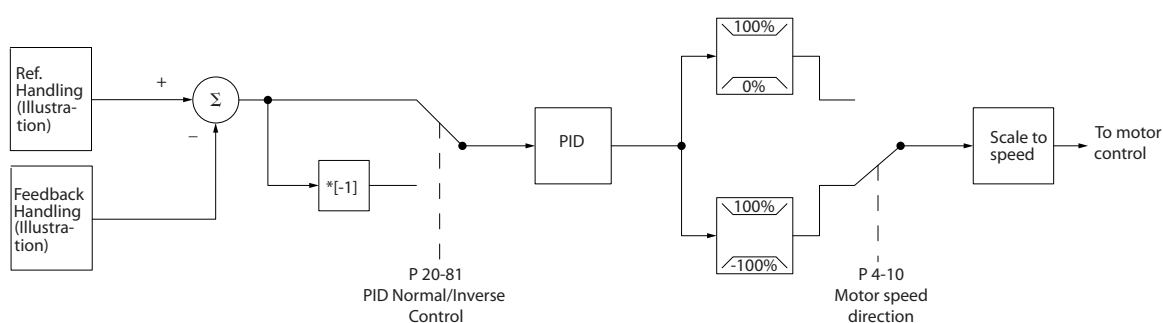
Figure 11.7 Block Diagram of Closed-loop Controller
