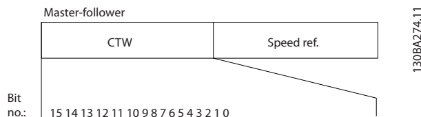
Figure 14.16 CW Master-to-Slave
