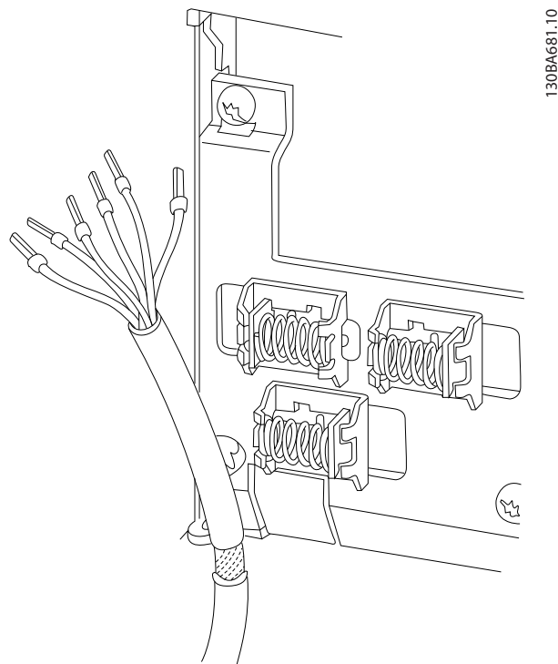
Figure 10.16 Shield Termination and Strain Relief of Control Cable
