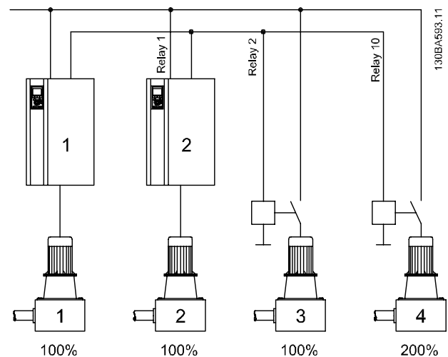
Figure 5.7 Application Overview
