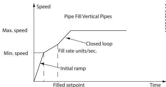
Figure 12.6 Performance Curve for Pipe Fill Mode
