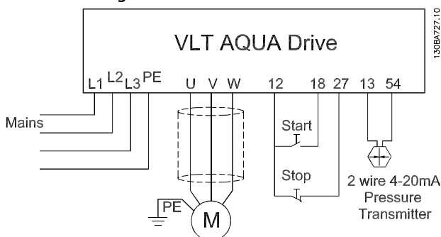
Figure 12.5 Wiring for Submersible Pump Application
