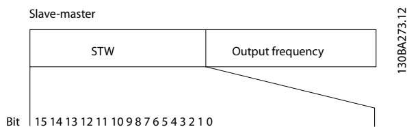
Figure 14.17 STW Slave-to-Master
