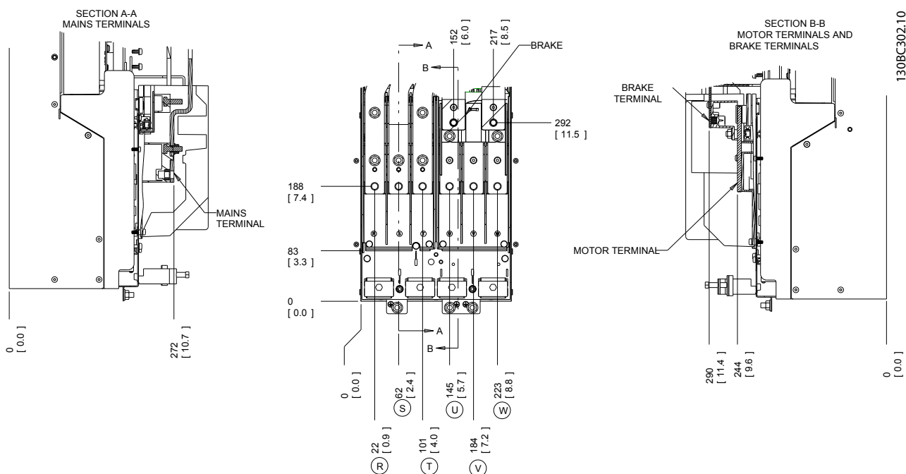
Illustration 4.7 Klemmeplaceringer, D3h
