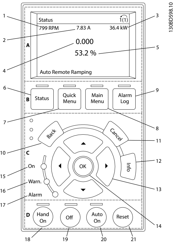
Illustration 5.1 LCP-betjeningspanel
