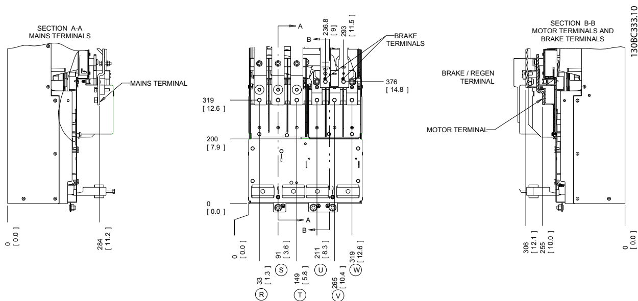
Illustration 4.9 Klemmeplaceringer, D4h
