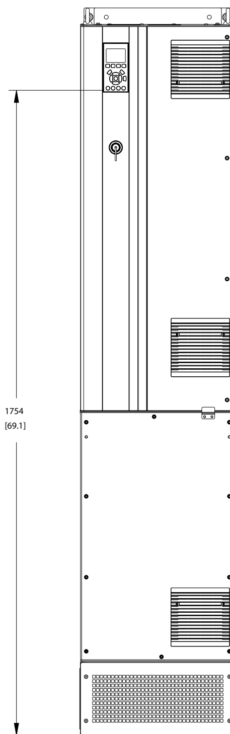
Illustration 1.2 D7h-kapsling
