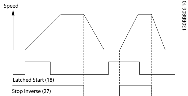
Figure 12.2 Latched Start/Stop Inverse
