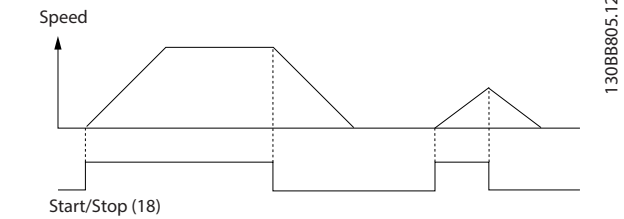
Figure 12.1 Start/Stop with Safe Torque Off
