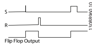
Illustration 3.52 Sorties bascules
