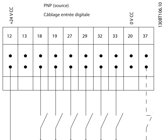
Illustration 1.3 PNP (source)
