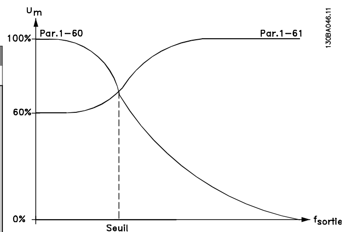
Illustration 3.11 Inversion
