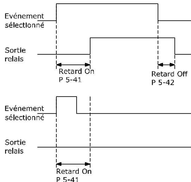
Illustration 3.35 Relais, retard ON
