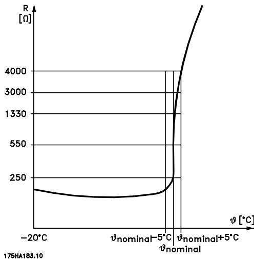
Illustration 6.1 Profil PTC
