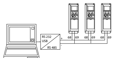
Illustration 5.8 Exemple de raccordement.
