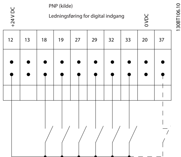
Illustration 3.52 PNP (kilde)
