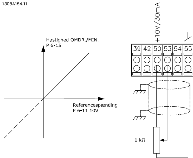
Illustration 3.59 Potentiometerreference
