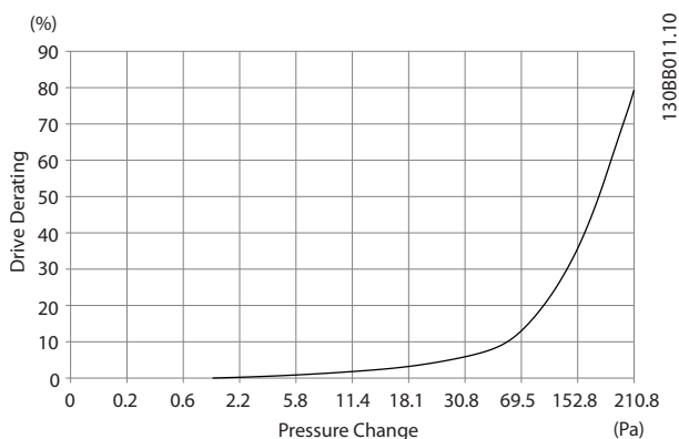
Figure 9.6 Derating vs. Pressure Change for E1-E2 Enclosures, 380–500 V Models: P315–P400 and 525–690 V Models: P500–P560. Airflow: 850 cfm (1445 m 3 /h)
