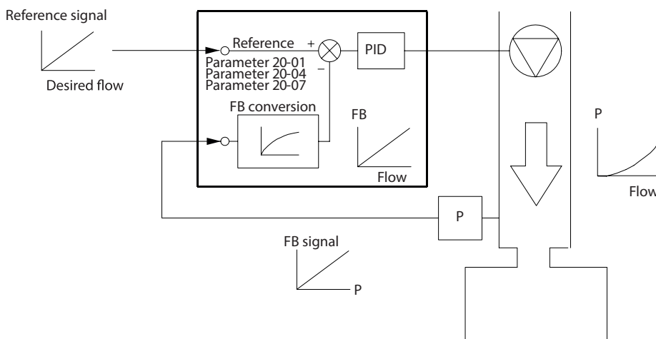
Figure 11.5 Feedback Conversion
