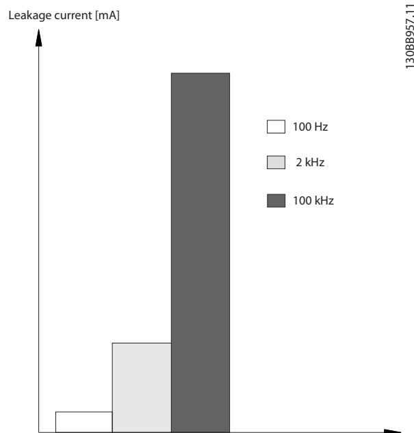
Figure 10.25 Influence of the RCD Cut-off Frequency on Leakage Current
