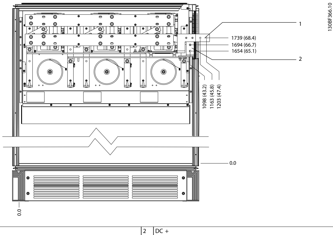
Figure 8.55 Terminal Dimensions for F2/F4 Regeneration Terminals, Front View
