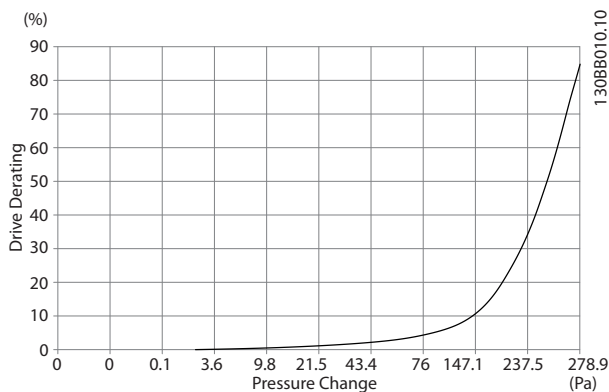
Figure 9.5 Derating vs. Pressure Change for E1-E2 Enclosures, 380–500 V Models: P250 and 525–690 V Models: P355–P400. Airflow: 650 cfm (1105 m 3 /h)
