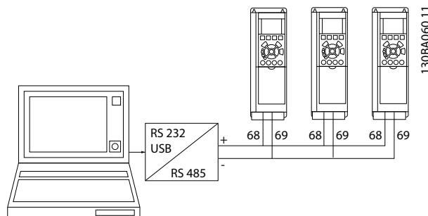
Figure 14.2 Parallel Connections
