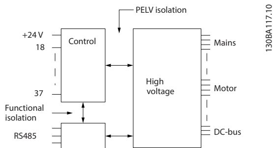
Figure 7.1 PELV Isolation
