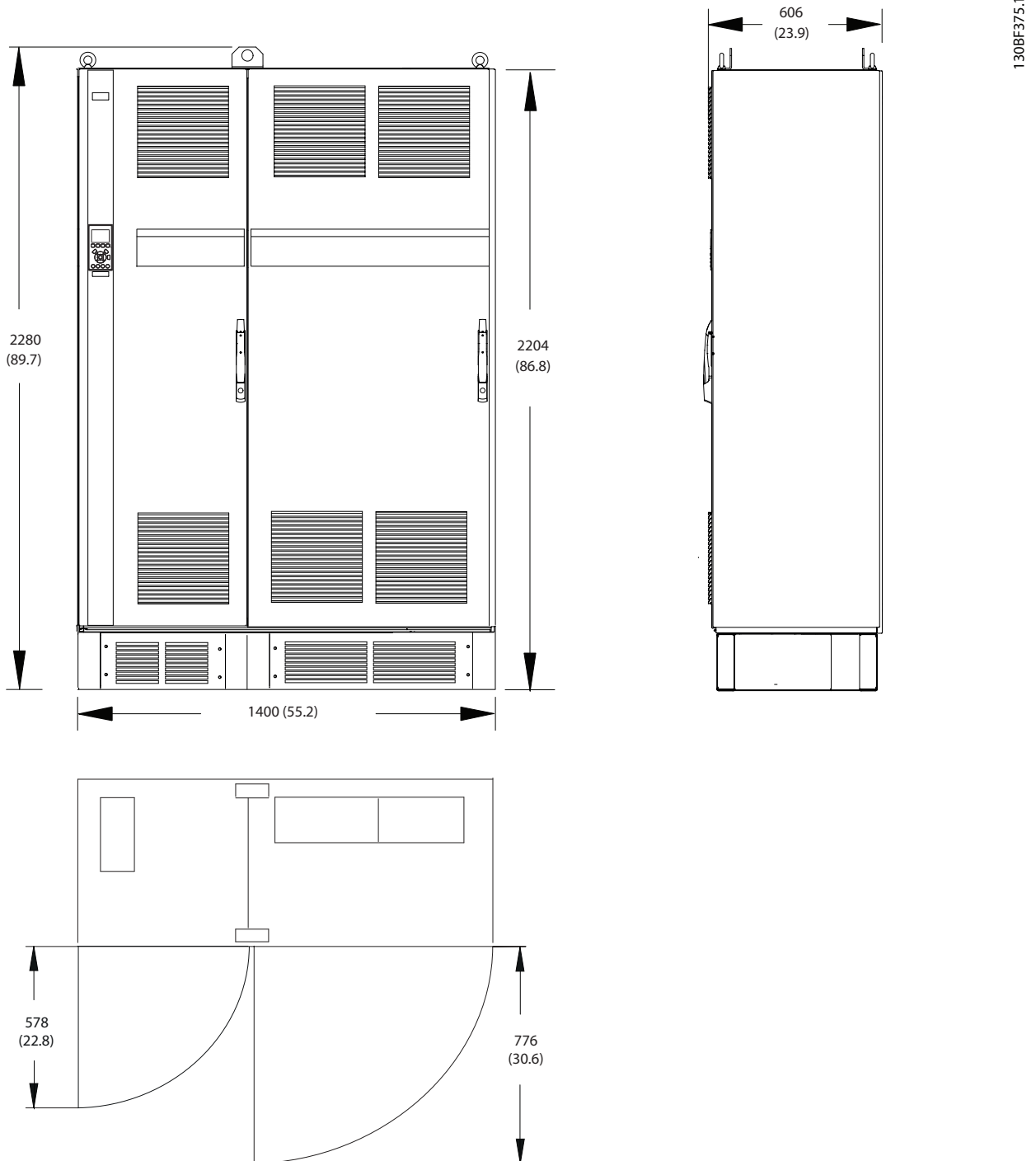
Figure 8.19 Front, Side, and Door Clearance Dimensions for F1
