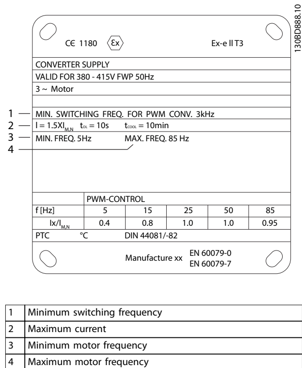
Figure 5.2 Motor Nameplate showing Drive Requirements
