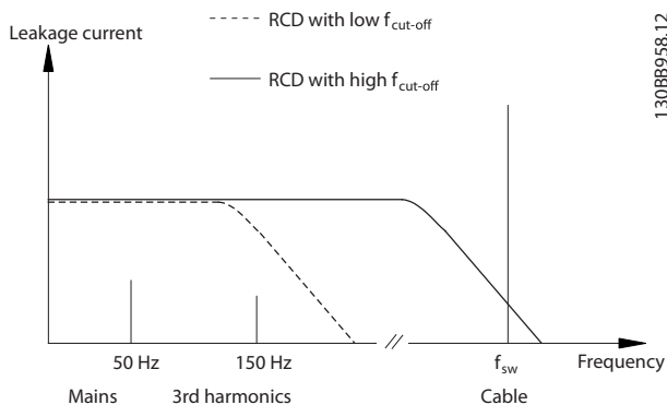
Figure 10.24 Main Contributions to Leakage Current
