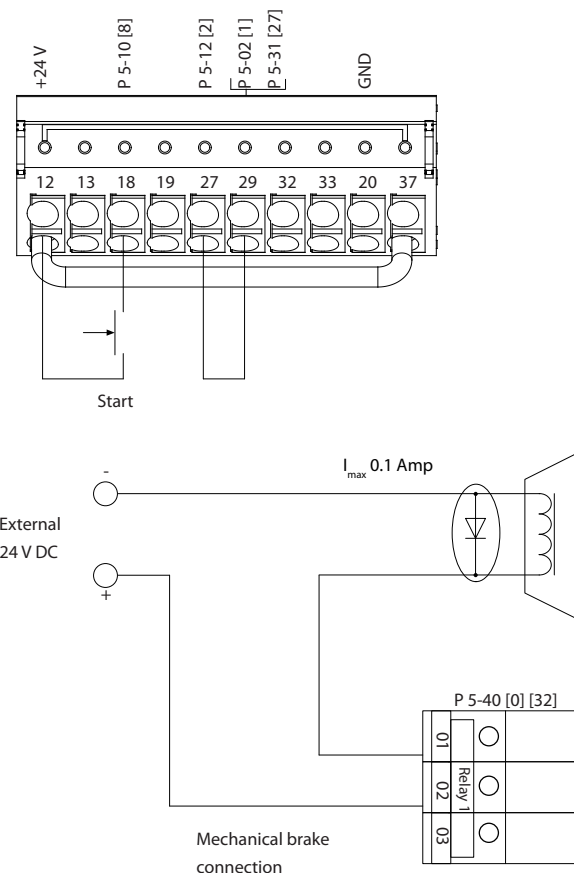
Figure 12.8 Wire Configuration for Torque and Stop Limit
