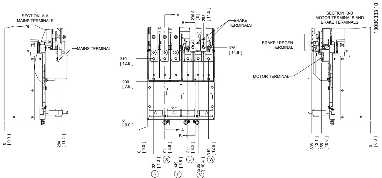
Illustration 2.10 Klemmeplaceringer D4h
