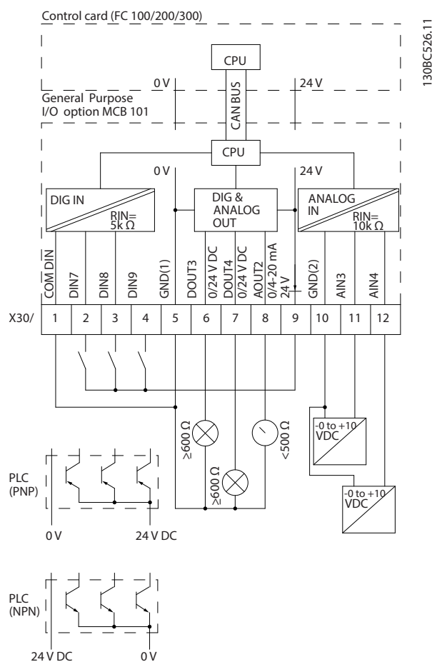
Illustration 7.5 Principle Diagram
