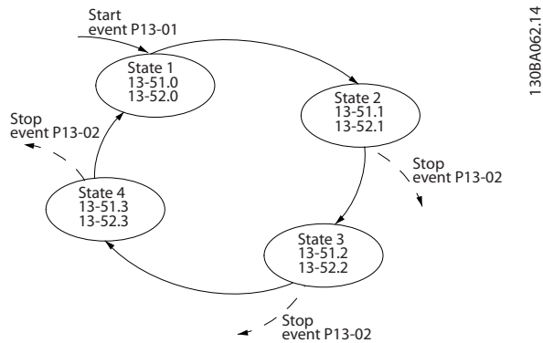
Illustration 14.9 Internal Current Control Example
