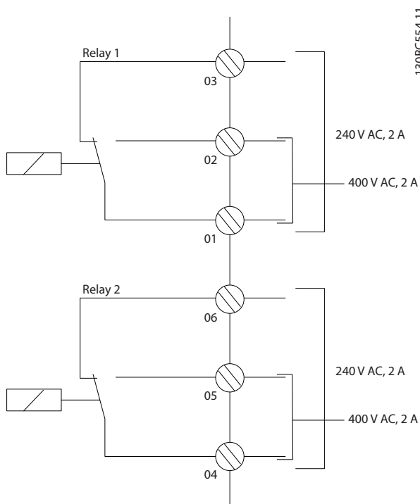
Illustration 12.5 Extra Relay Outputs
