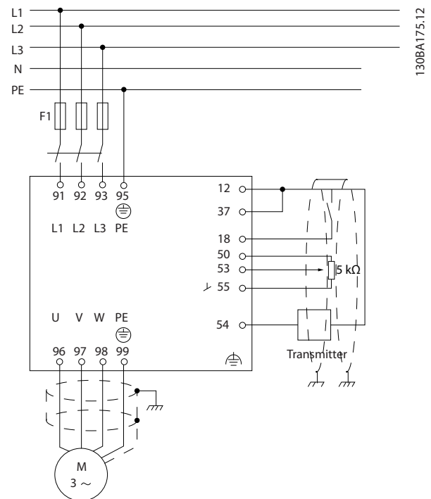
Illustration 16.4 Two-wire Transmitter
