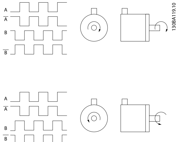
Illustration 7.8 Rotation Direction
