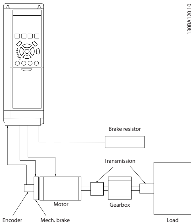
Illustration 17.7 Basic Set-up for FC 302 closed-loop Speed Control
