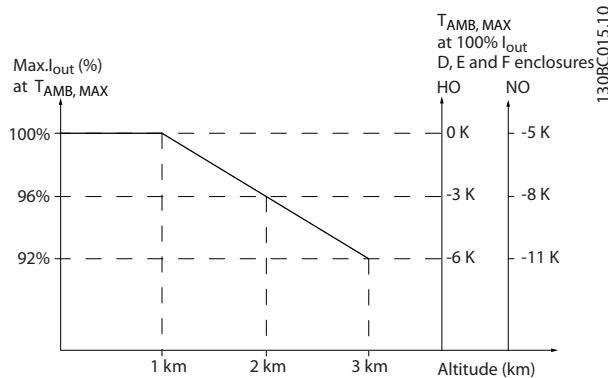
Illustration 6.19 Derating of Output Current Based on Altitude at T_{AMB,MAX}
