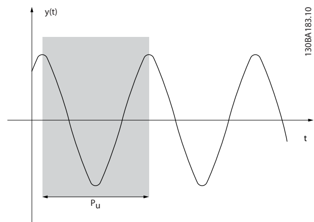
Illustration 16.5 Marginally Stable System
