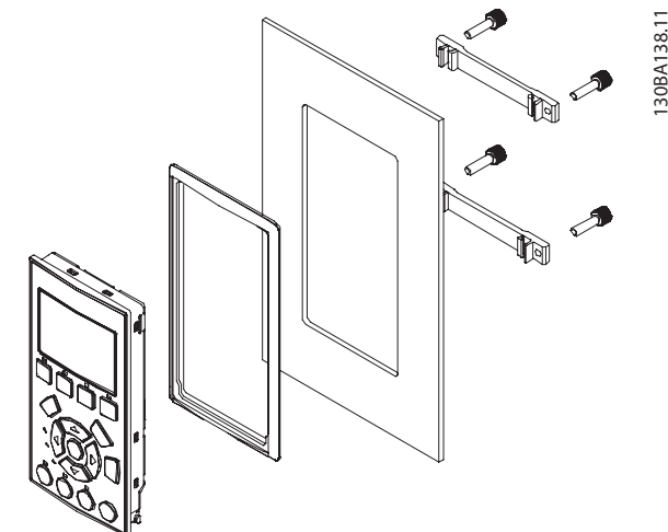
Illustration 7.19 Ordering Number 130B1113, LCP Kit with Graphical LCP, Fasteners, Cable, and Gasket
