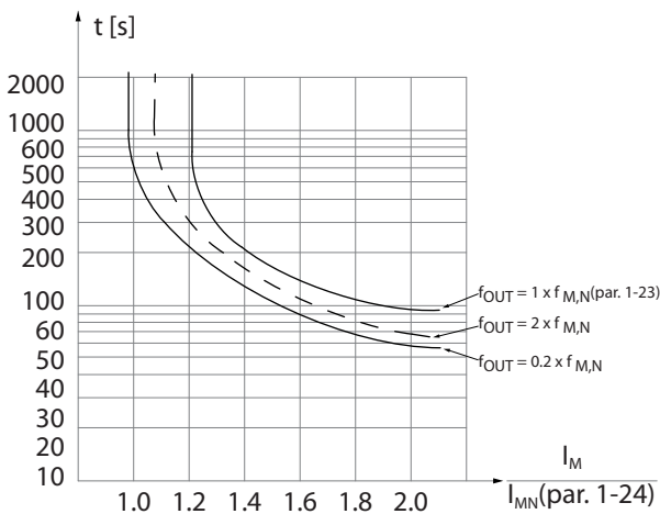
Illustration 10.11 ETR Example
