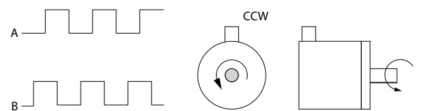
Illustration 17.6 24 V Incremental Encoder. Maximum Cable Length 5 m (16 ft)
