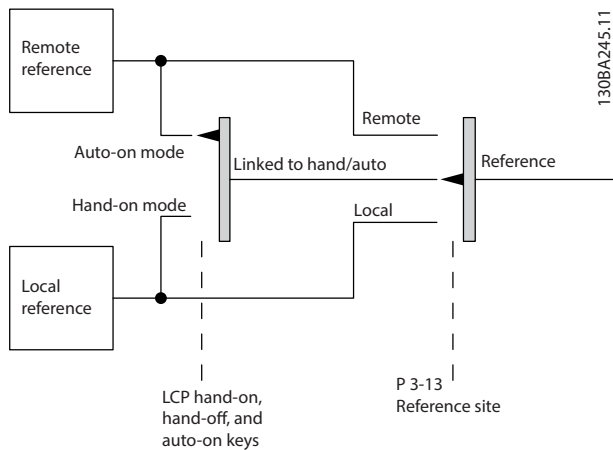
Illustration 14.6 Active Reference
