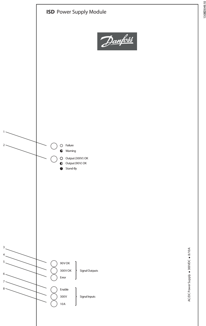
Illustration 8.2 LEDs
