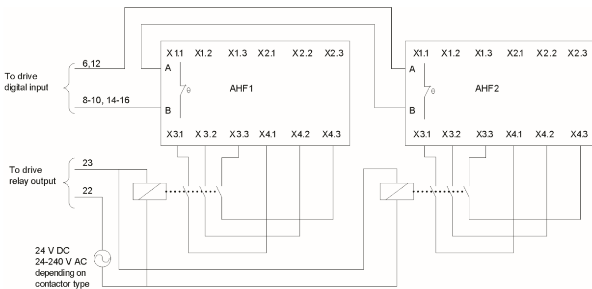
Figure 2. Parallel use of two AHF filters with capacitor disconnection
