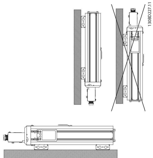
Illustration 9.23 Mechanical Mounting
