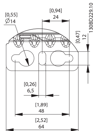
Illustration 9.20 Mounting Hole
