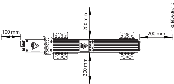
Illustration 3.7 Horizontal Mounting, IP21 and IP65 Versions with Connection Box
