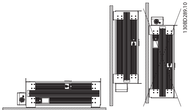
Illustration 9.90 Mechanical Mounting
