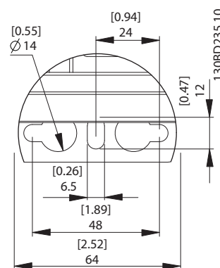
Illustration 9.14 Mounting Hole
