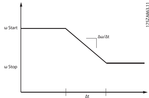
Illustration 4.3 Braking of High Inertia
