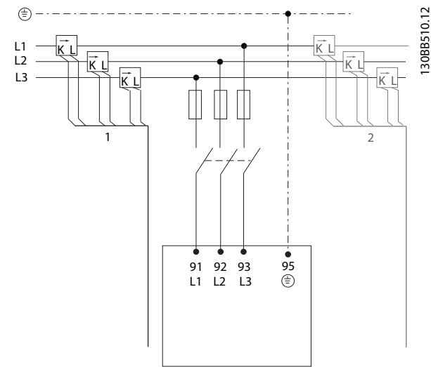
Illustration 4.5 Raccordements des TC
