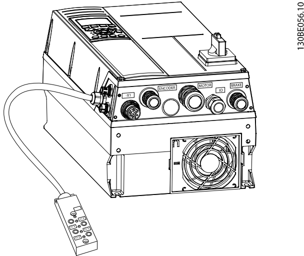
Illustration 3.3 Mains Connectors and 4 Cable Glands
