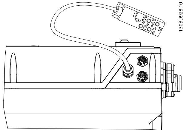
Illustration 3.4 Side View
