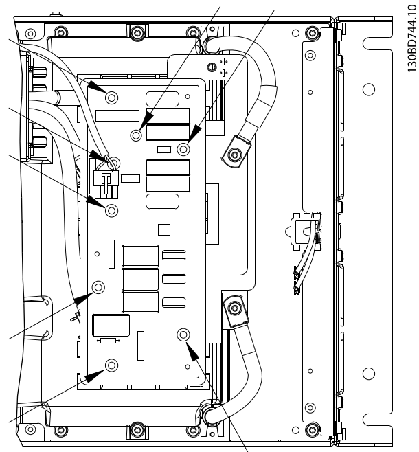
Illustration 1.2 Positions of M4 Screws on RFI Auxiliary Card, Enclosure Type J7
