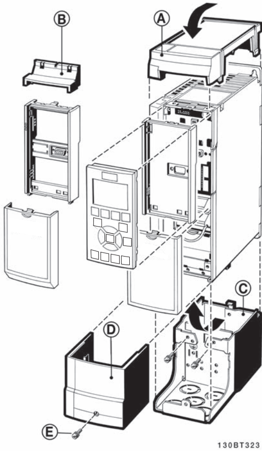
Illustration 1.1 TR200 (230 V, 1 to 3 HP, 460 V, 1 to 5 HP)
