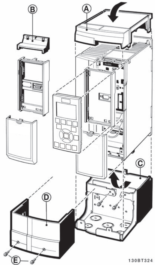
Illustration 1.2 Frame Size A3 TR200 (230 V, 5 HP, 460 V, 7.5 to 10 HP, 575 V 1 to 10 HP)
