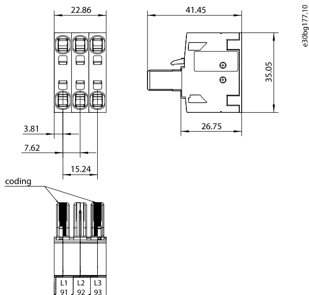
Illustration 1.1 Double Push-in Mains Connector/Terminal Block
