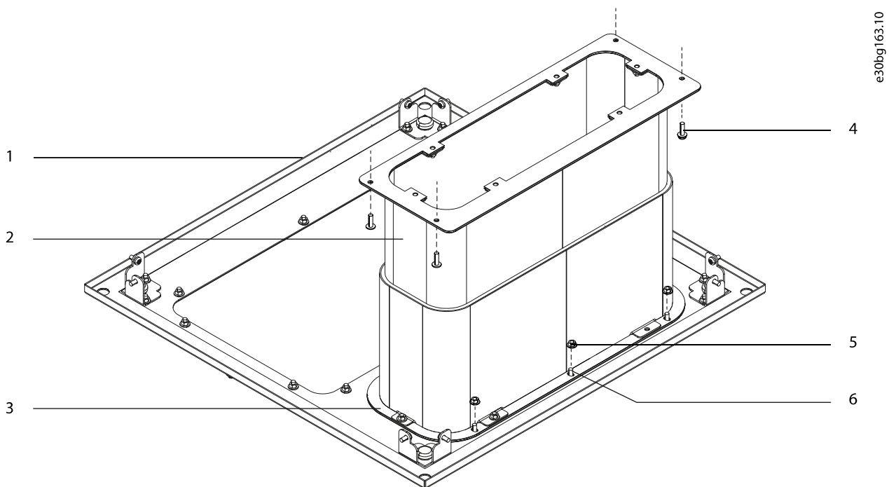
Illustration 1.8 Installation of the Bottom Duct on the Base Plate
