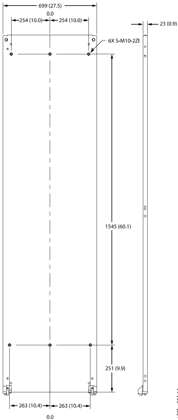
Illustration 1.3 Mounting Plate in 800 mm (32 in) Enclosure
