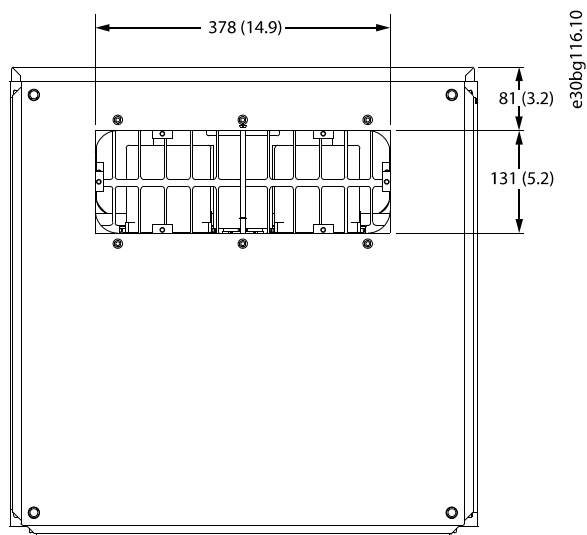
Illustration 1.4 Dimensions of Vent in Top of Drive
