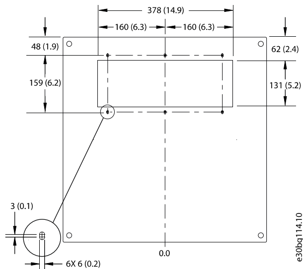
Illustration 1.5 Dimensions for Opening in Enclosure Top Plate
