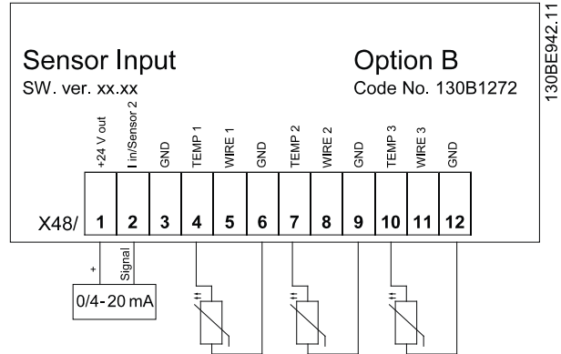
Illustration 1.4 2-Wire Sensors
