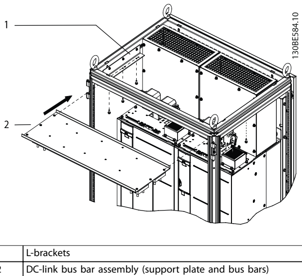
Illustration 1.3 Installation of DC Bus Bars onto L-brackets
