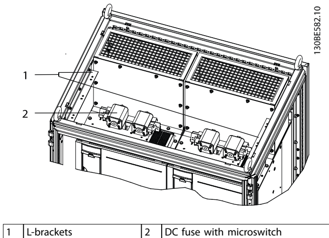
Illustration 1.1 Installation of DC Bus Bar L-brackets above the DC Fuses
