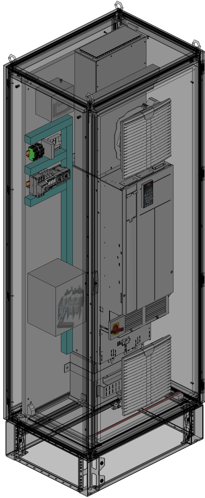
3D mounting layout 3D-Montageaufbau
