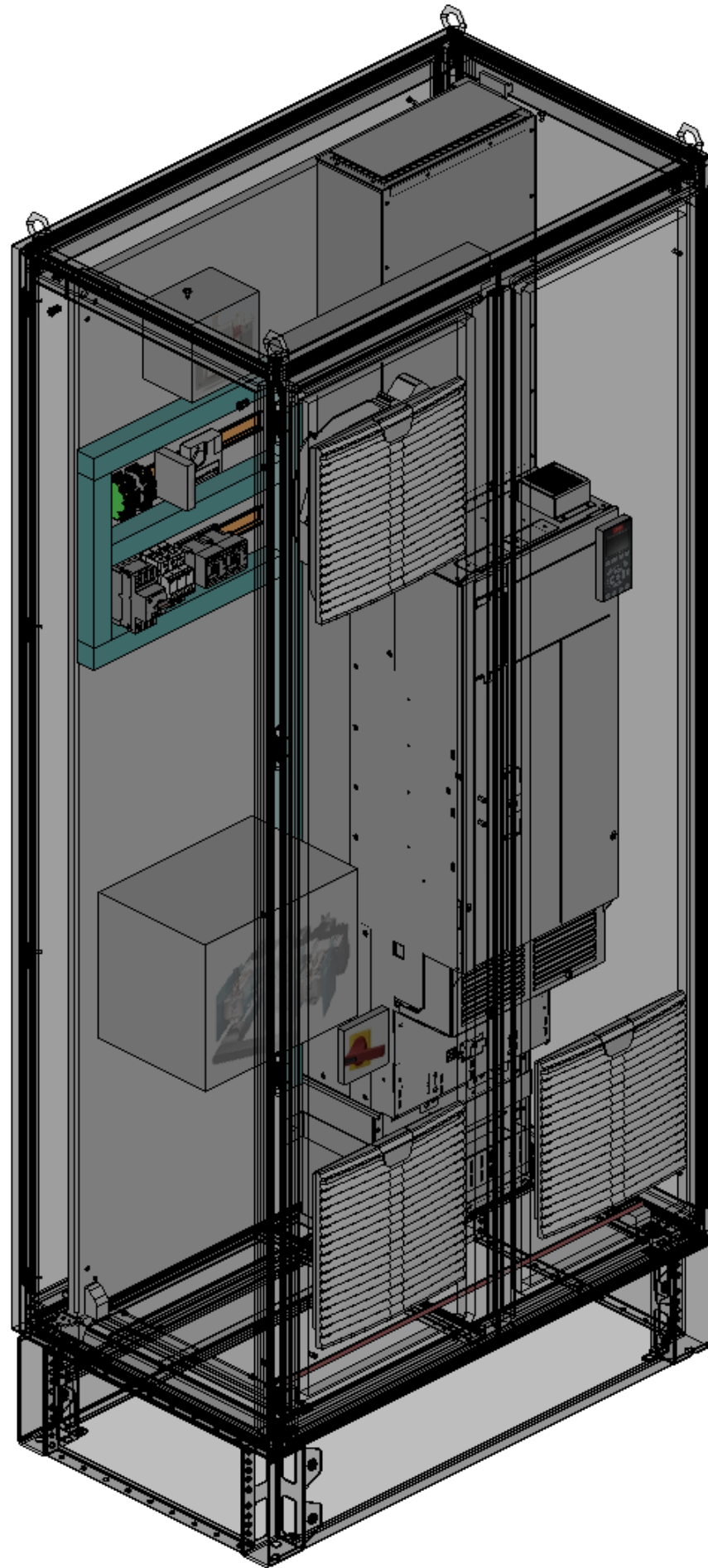
3D mounting layout 3D-Montageaufbau
