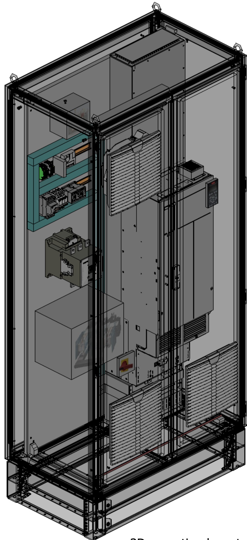
3D mounting layout 3D-Montageaufbau
