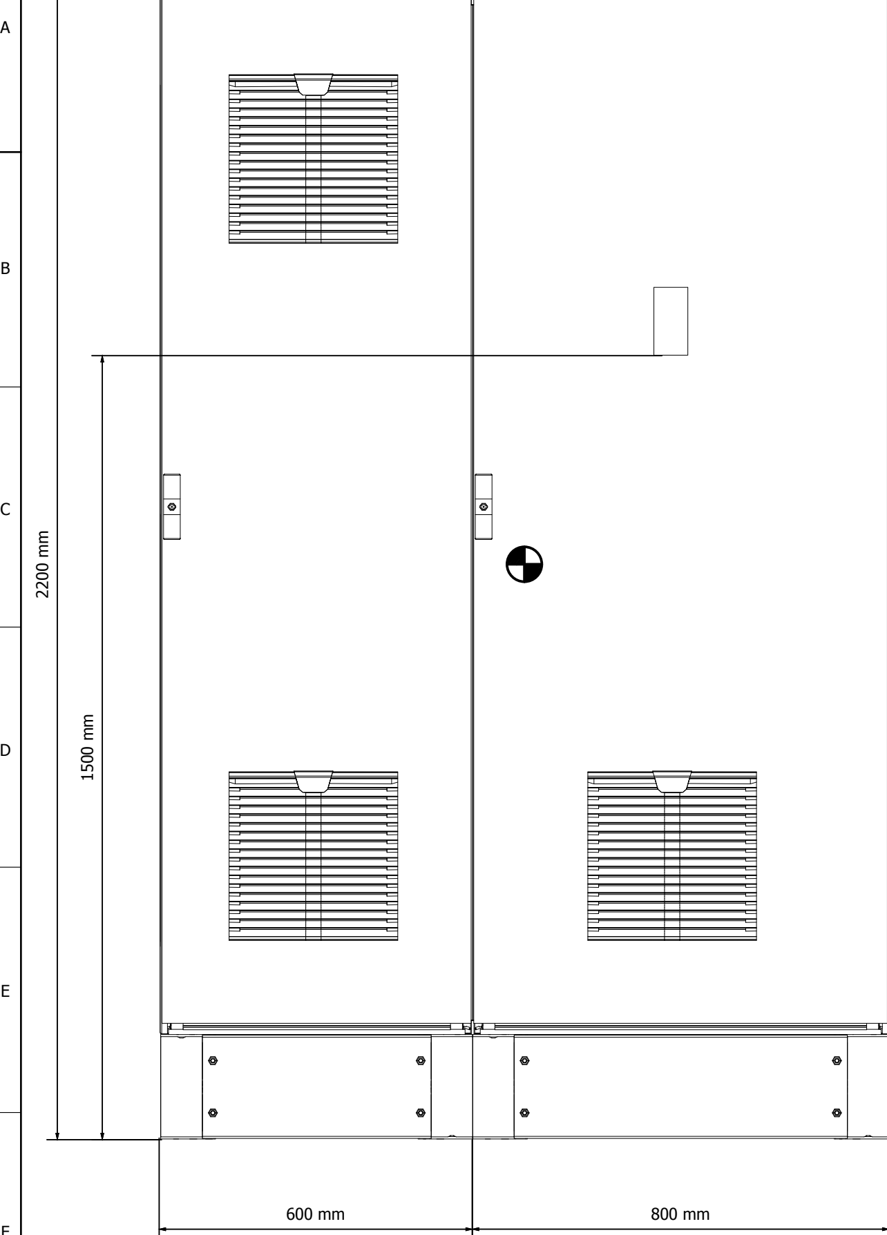
Front view Frontansicht
