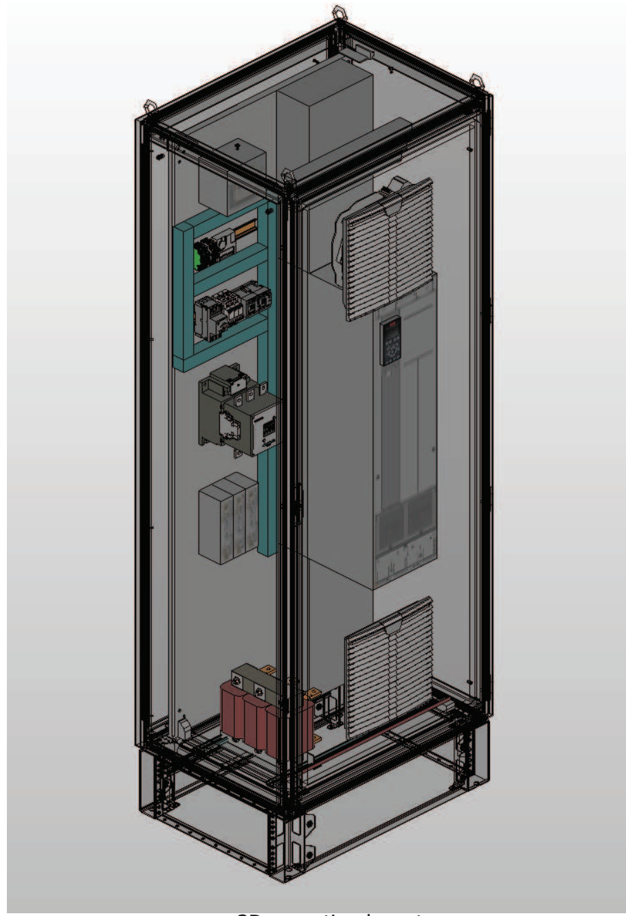
3D mounting layout 3D-Montageaufbau
