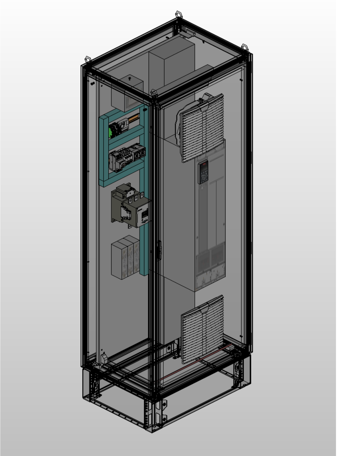
3D mounting layout 3D-Montageaufbau
