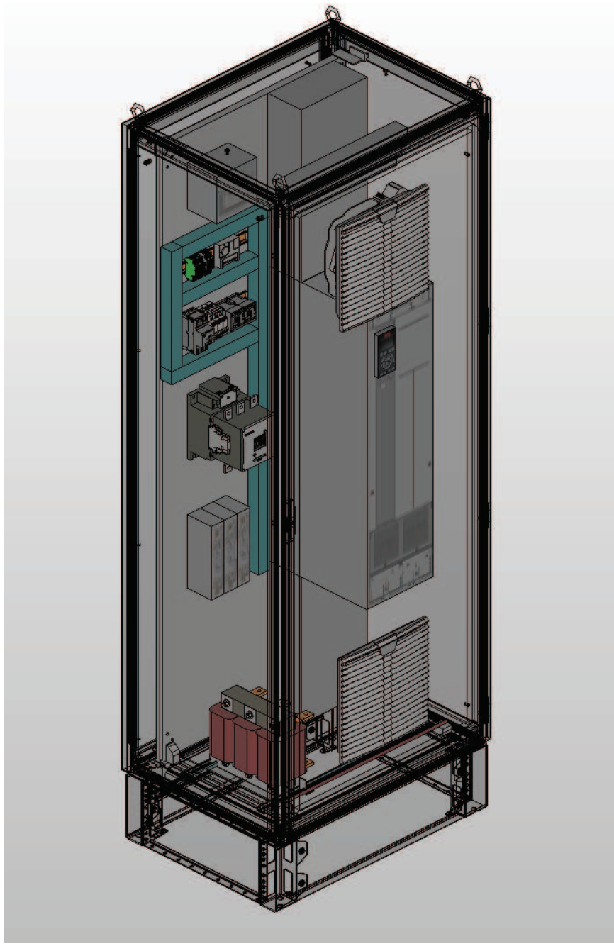
3D mounting layout 3D-Montageaufbau
