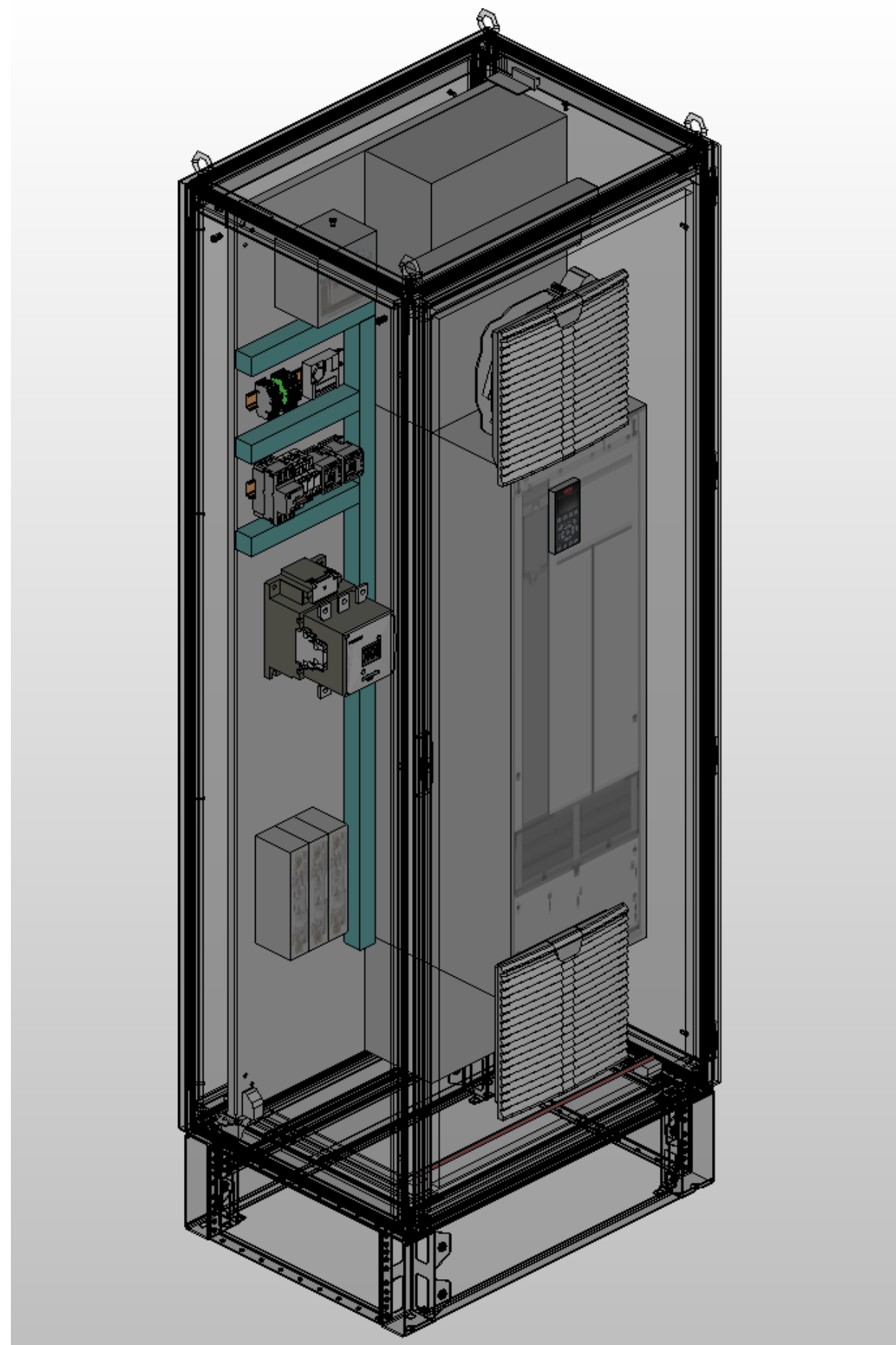
3D mounting layout 3D-Montageaufbau
