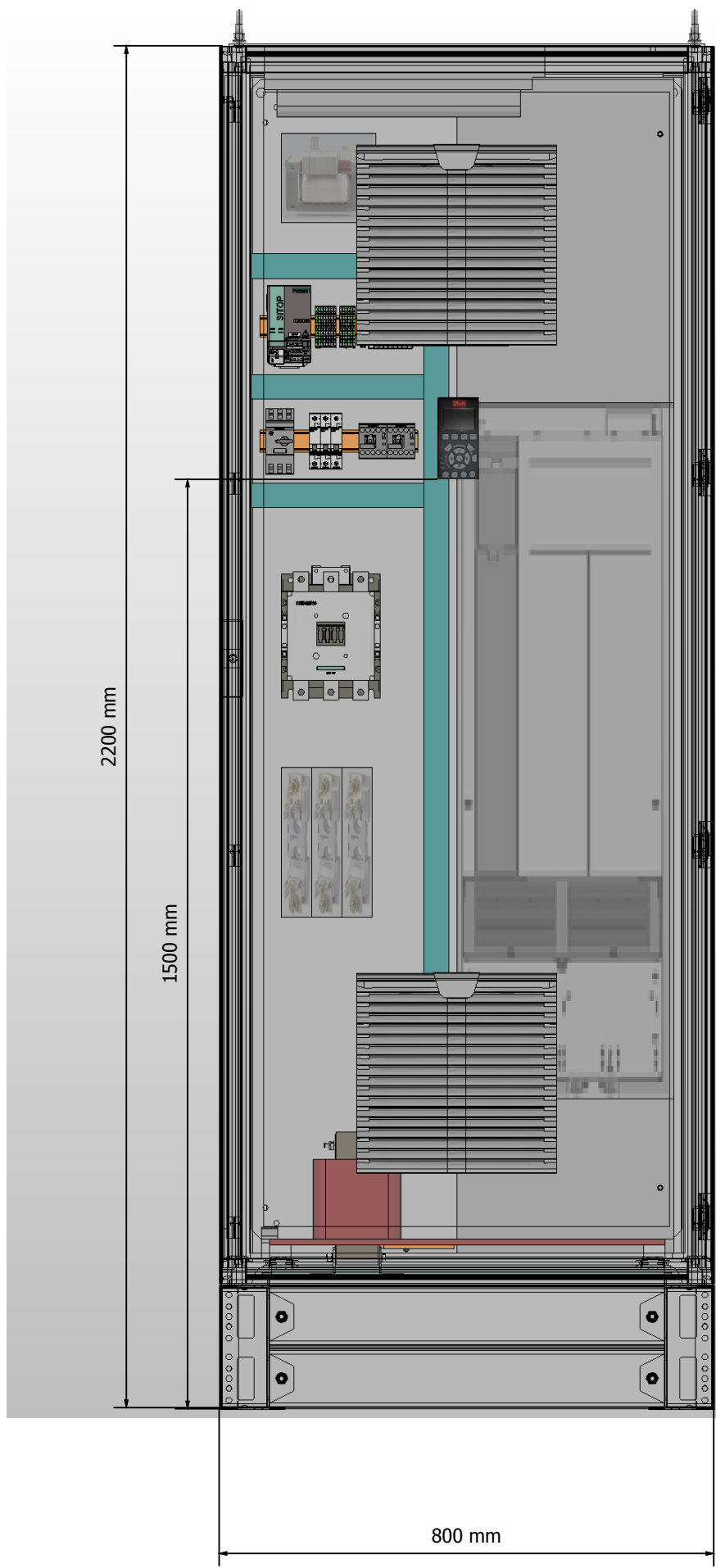
Front view Frontansicht
