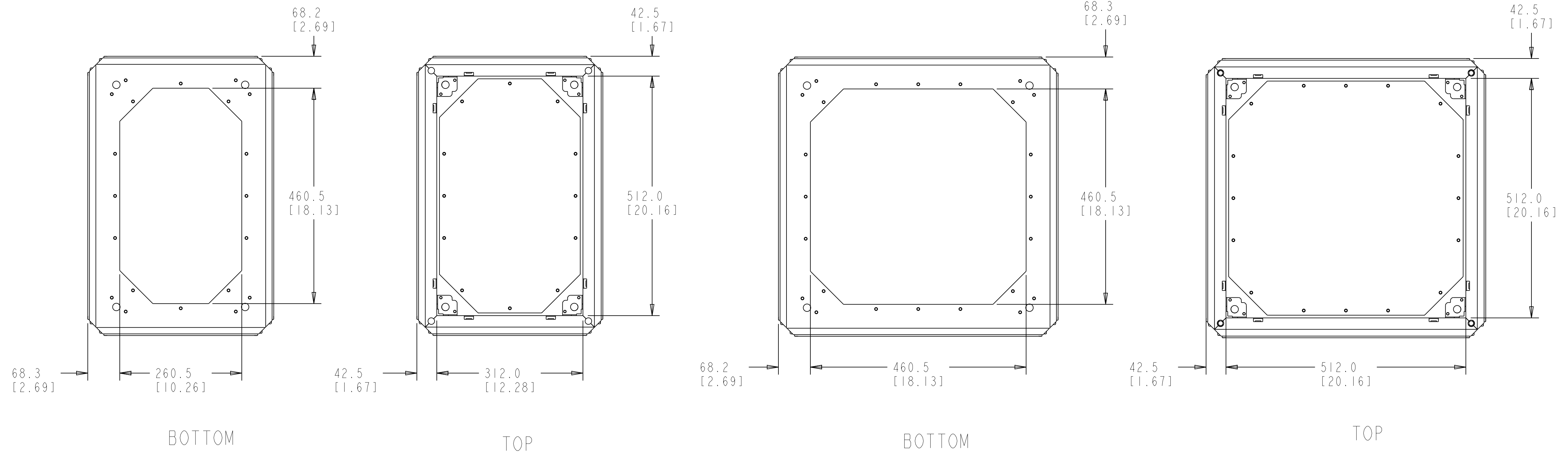
400MM CABINET
