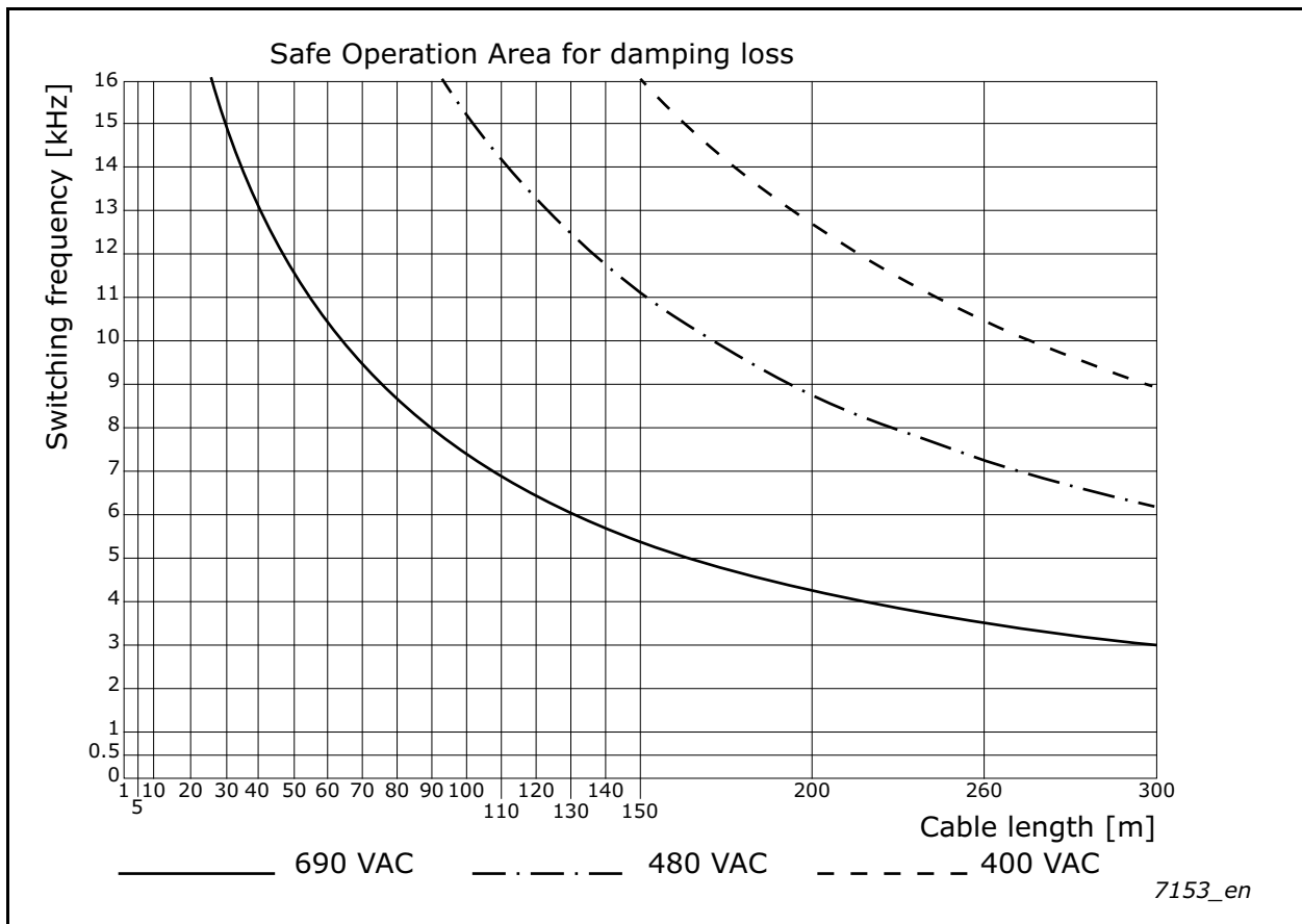
Figure 40. Safe operating area for DUT-1250-6-0-S and DUT-1600-6-0-S
