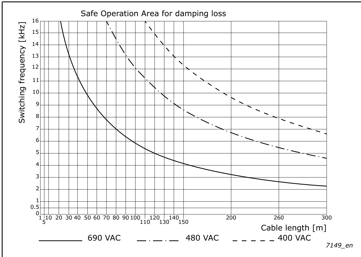
Figure 36. Safe operating area for DUT-0280-6-0-S
