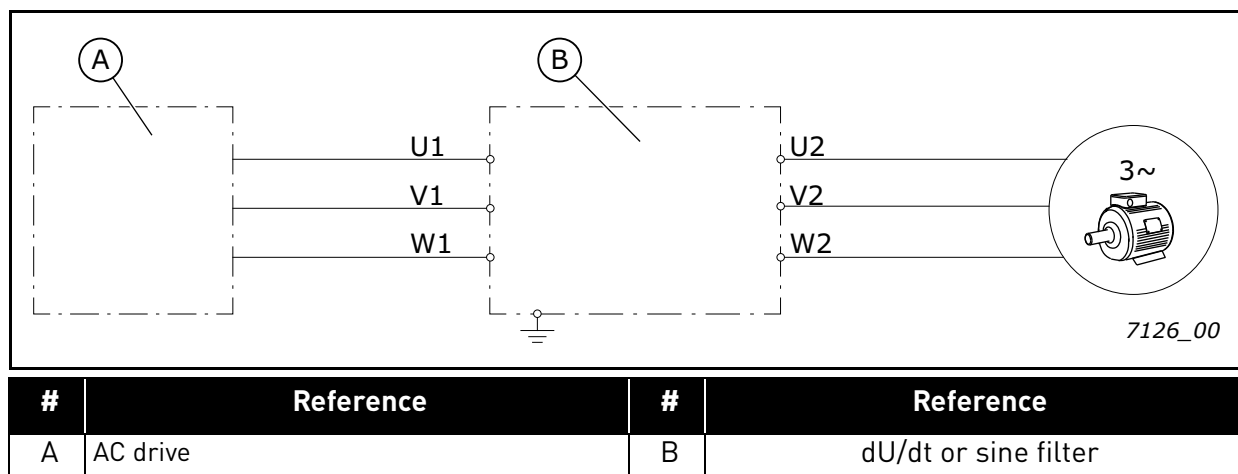
Figure 9. Filter connection
