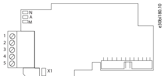
Illustration 52: LED Indications on VACON® OPTC7 Option Board
