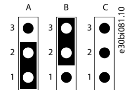
Illustration 18: The Settings of the Jumper X6 on Board, Termination Resistor, Positions A, B, and C
