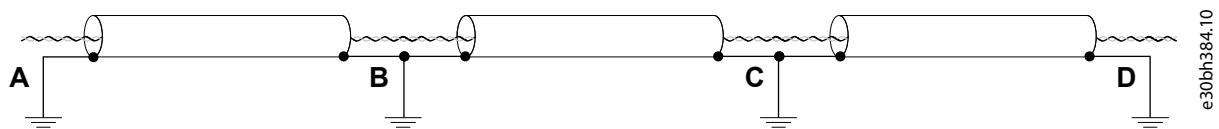
Illustration 9: Grounding in noisy environment with good equipotential. If potentials at points A, B, C and D are very different and cannot be made similar, cut the shields as in Illustration Grounding in noisy environment with poor equipotential.
