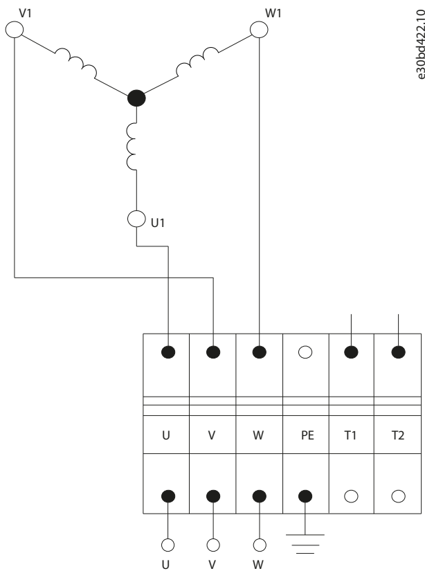
Illustration 9: Raccordement CAGE CLAMP®
