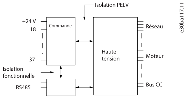
Illustration 51: Isolation PELV
