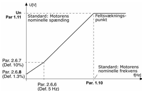
Figur 9.2: Programmerbar U/f-kurve
