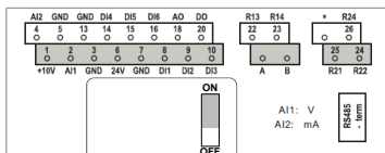
Figur 3.1: Vacon 10 I/O
