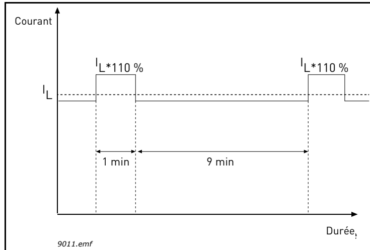
Figure 60. Faible surcharge
