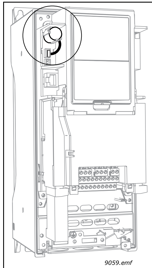
Figure 56. Optional battery
