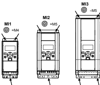
Figur 1: Skruvmontering, MI1–MI3
