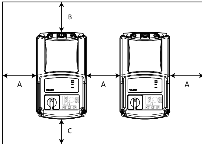
Figure 8. Installation space.
