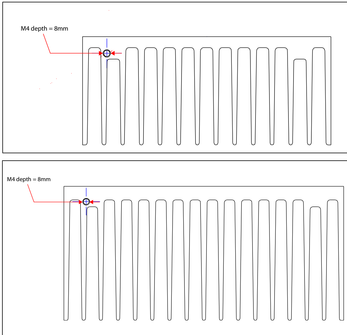
Figure 2. SECOND Protective Earth connection, MU3.
