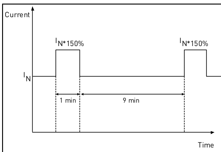
Figure 20. High overload.
