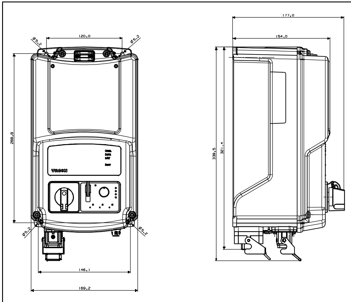
Figure 6. VACON® 20 X, MU2.
