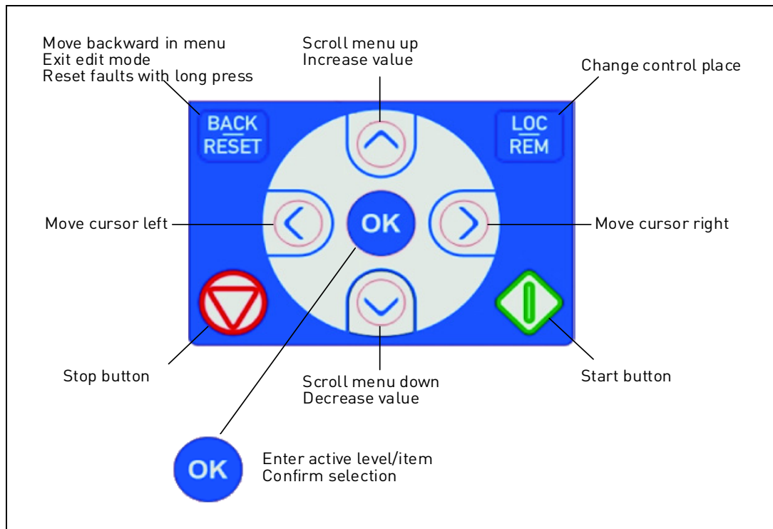
Figure 26. Keypad buttons.
