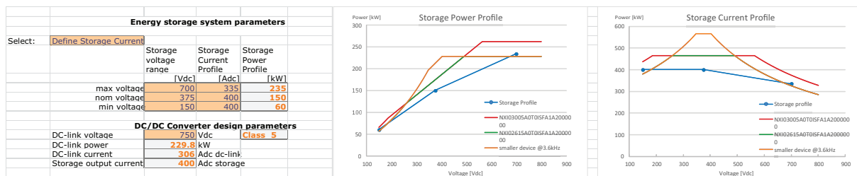
Figure 48. Power unit selection tool example based on storage power profile
