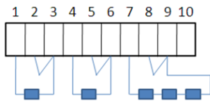
Two-wire configuration
