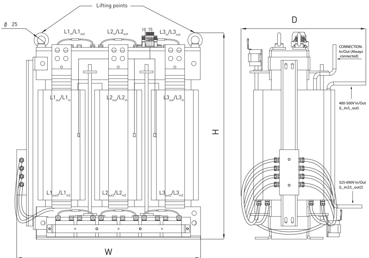
Figure 88. Example of L_{net} choke of a VACON® RLC filter
