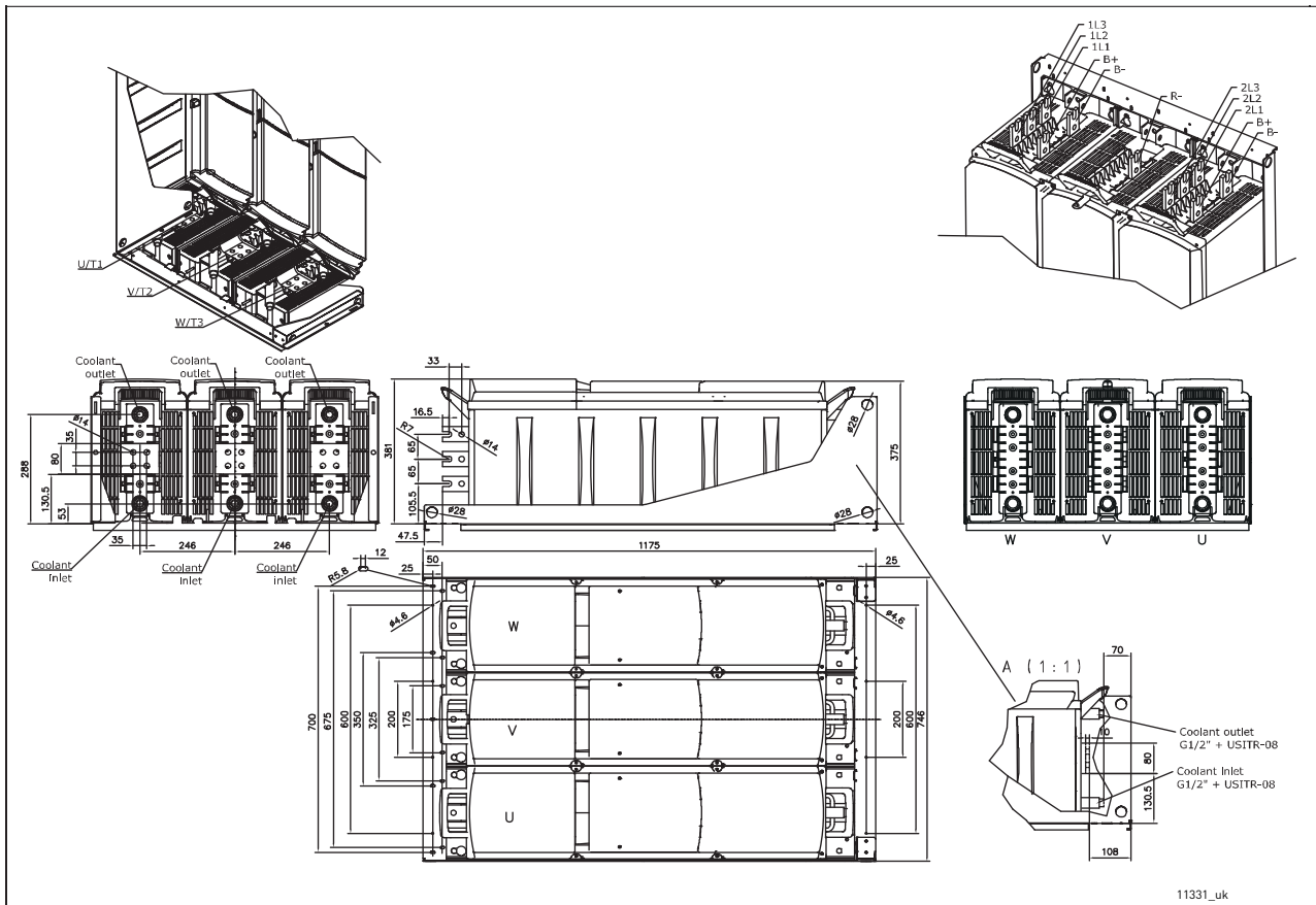
Figure 23. VACON ® NX Liquid-Cooled AC drive (12-pulse) with internal brake chopper dimensions, CH74, IP00
