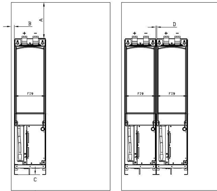
Figure 5-5. Installation space for F19.
