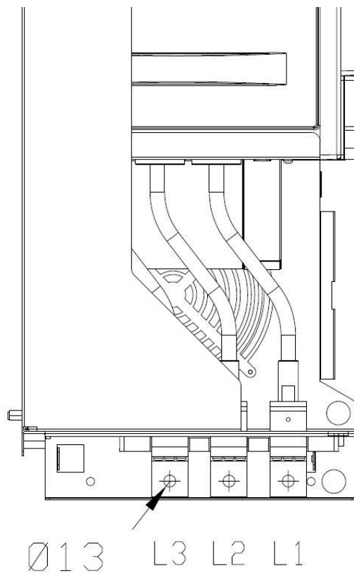
Figure 5-11. F19 unit AC connection.
