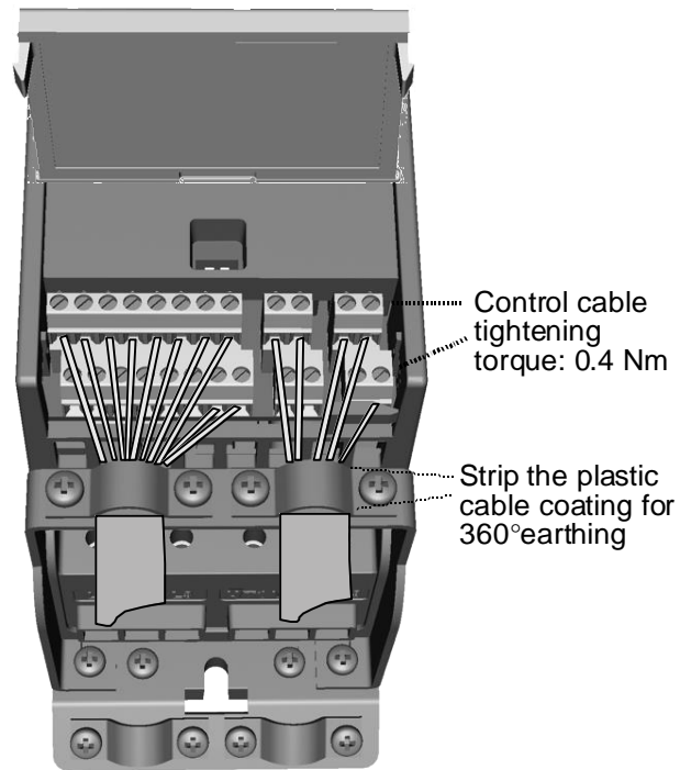
Figure 5-15. Cabling.
