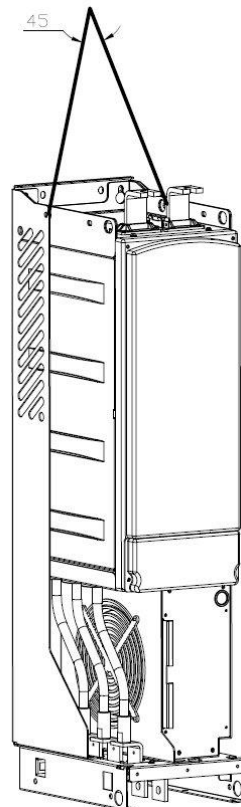
Figure 3-3. Lifting points for F19 module.
