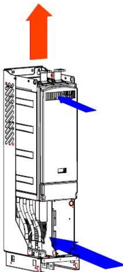
Figure 5-6. Cooling airflow for F19 NFE unit.
