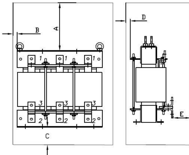
Figure 5-7. Installation space.
