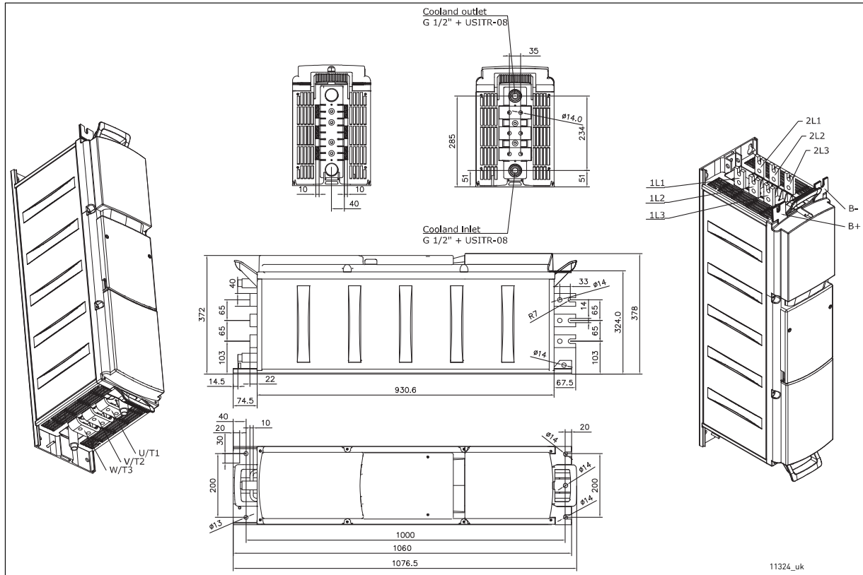
Figure 16. Vacon Liquid-Cooled frequency converter (12-pulse), CH72
