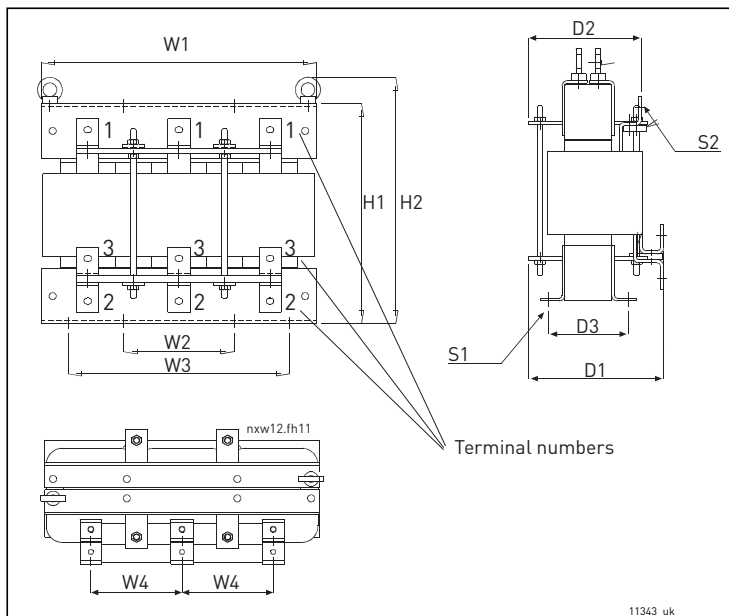
Figure 35. Example of input chokes for Vacon NX Liquid-Cooled. Sizes 261 A...1150 A 11343_uk
