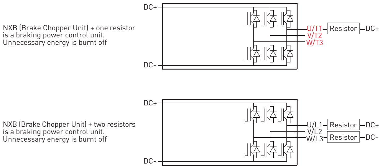
Figure 99. Brake chopper unit topology
