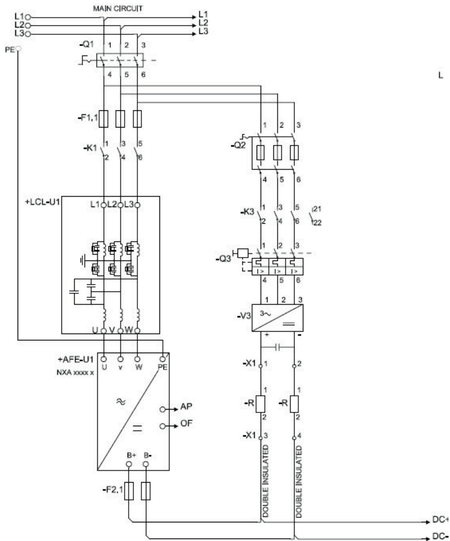
Figure 85. Active front end configuration
