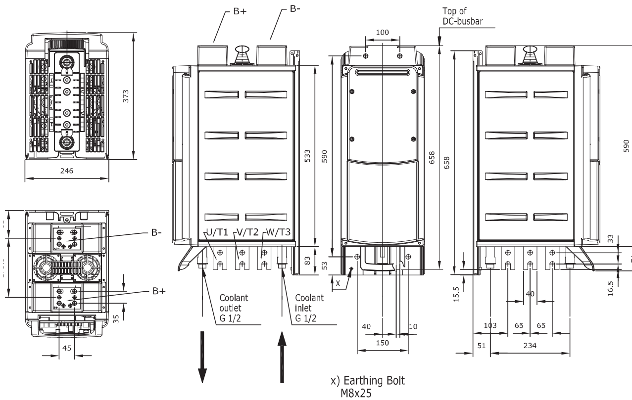
Figure 12. Vacon Liquid-Cooled inverter, CH61
