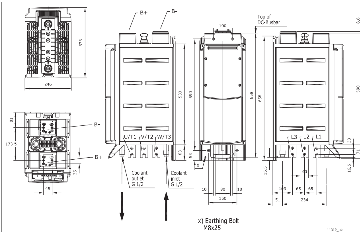
Figure 11. Vacon Liquid-Cooled frequency converter, CH61
