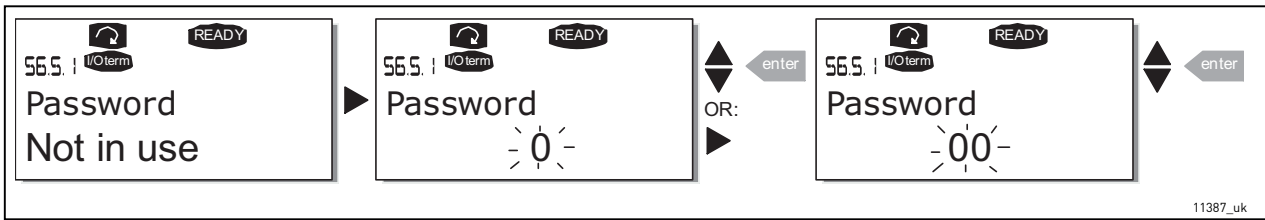
Figure 73. Password setting
