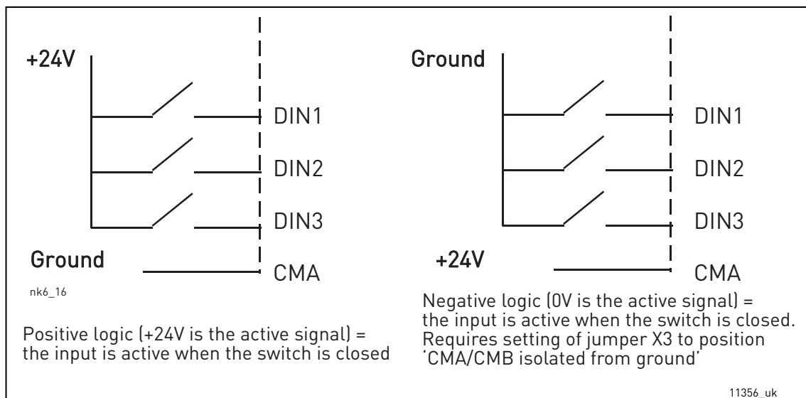
Figure 47. Positive/Negative logic
