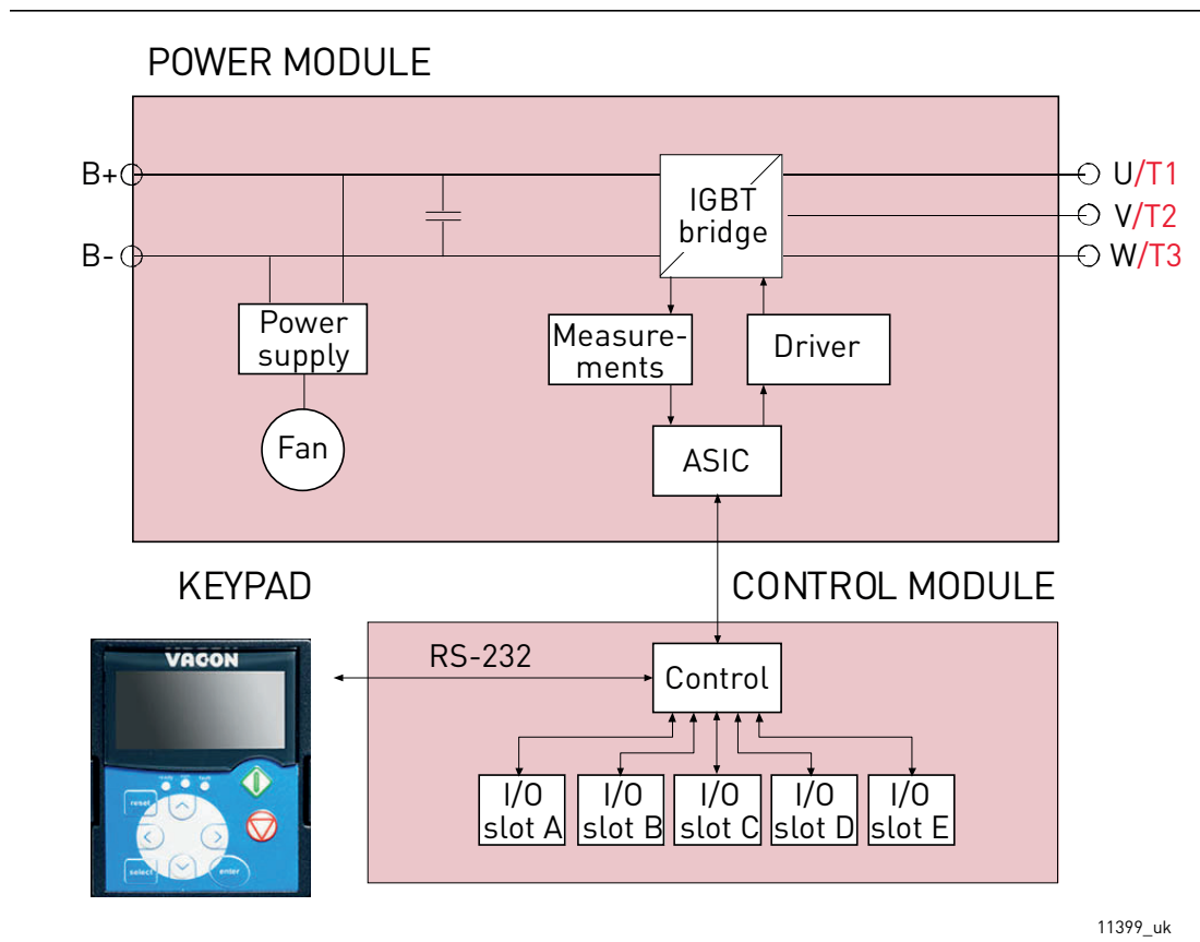
Figure 98. BCU block diagram
