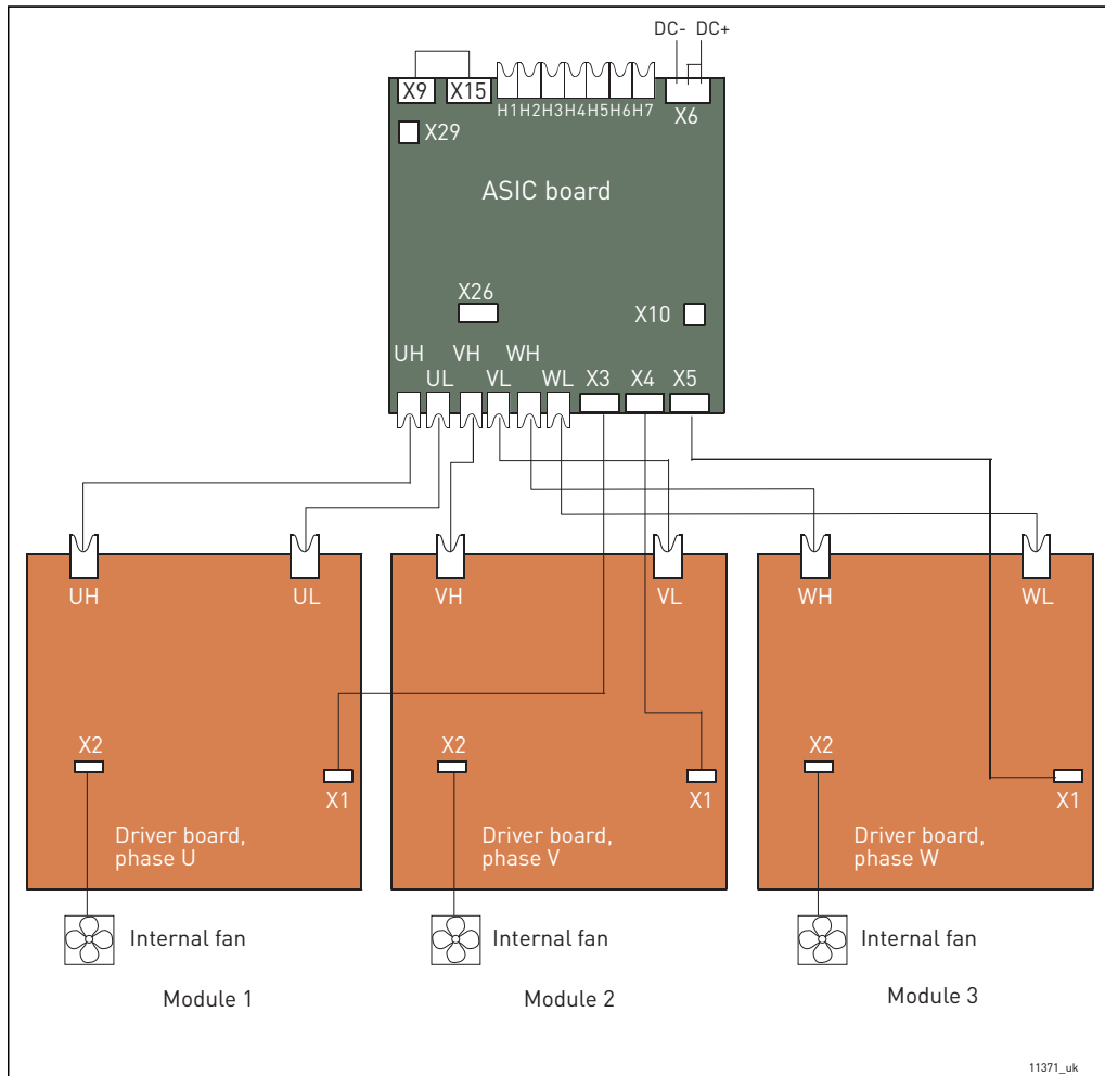
Figure 54. Terminals and connections between ASIC and driver boards (CH64 and CH74)
