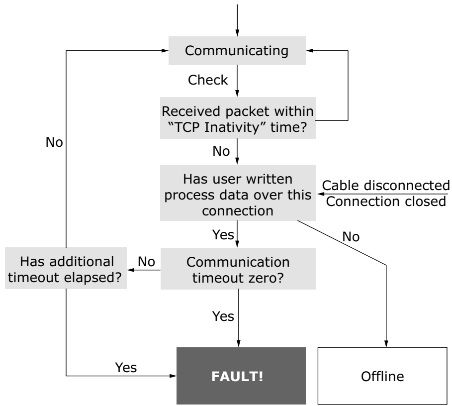
Figure 45. EtherNet/IP timeout logic with explicit connection
