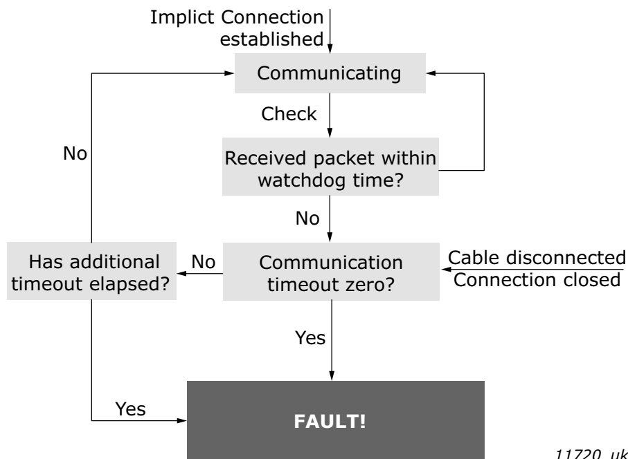
Figure 44. EtherNet/IP timeout logic with implicit connection (IO connection)
