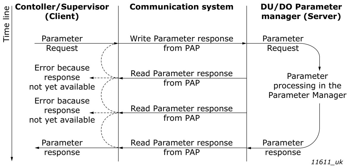
Figure 37. PROFdrive parameter access model
