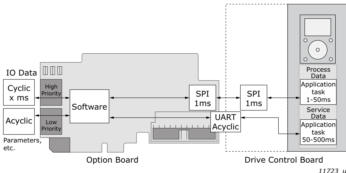
Figure 50. Fast fieldbus communication
