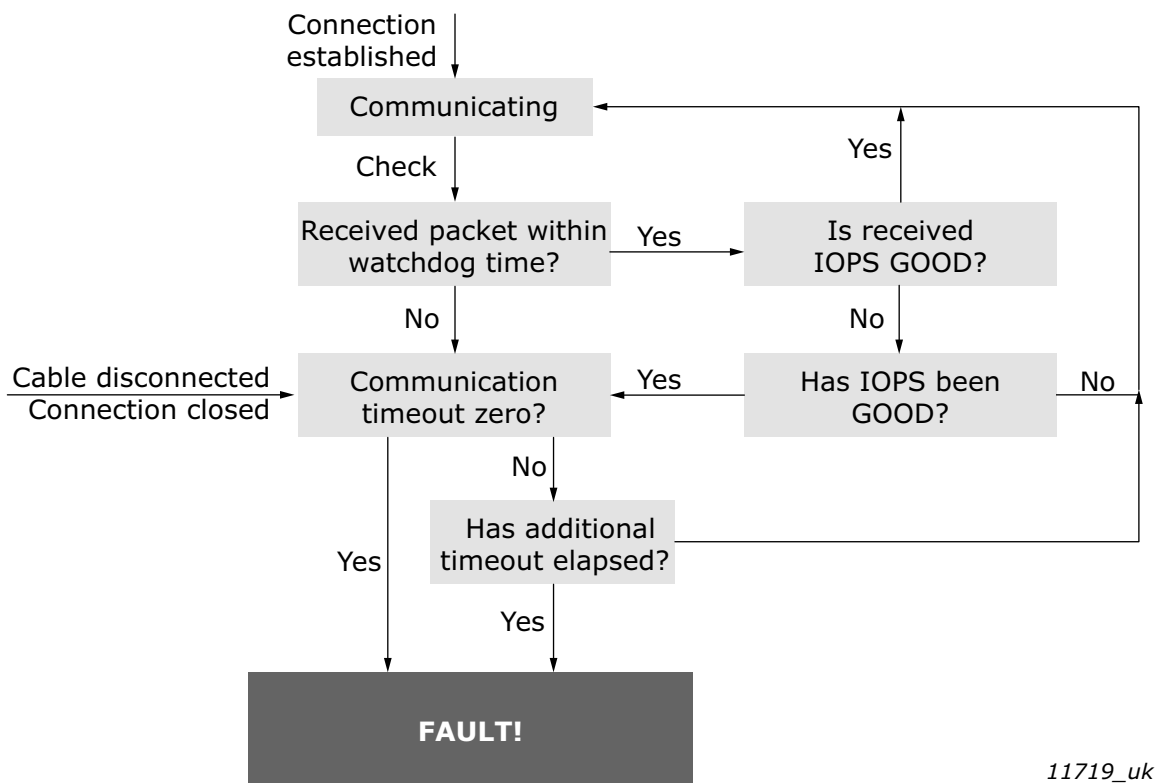
Figure 41. PROFINET IO communication and timeout fault
