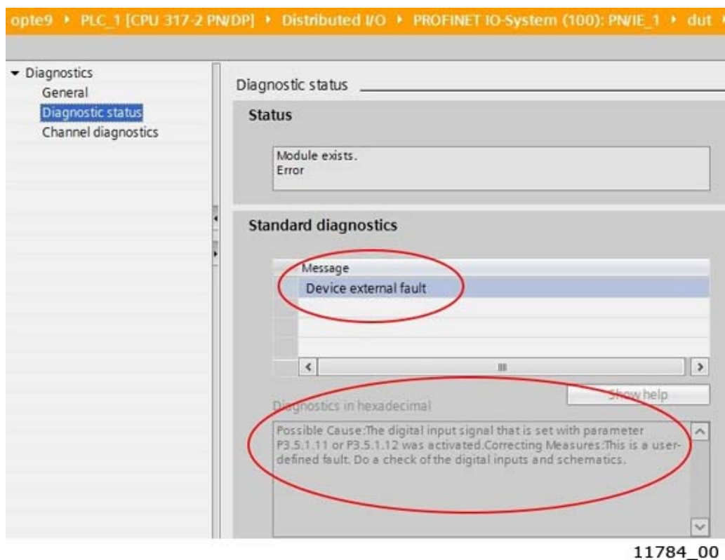
Figure 43. Siemens TIA portal - Alarm description and help text
