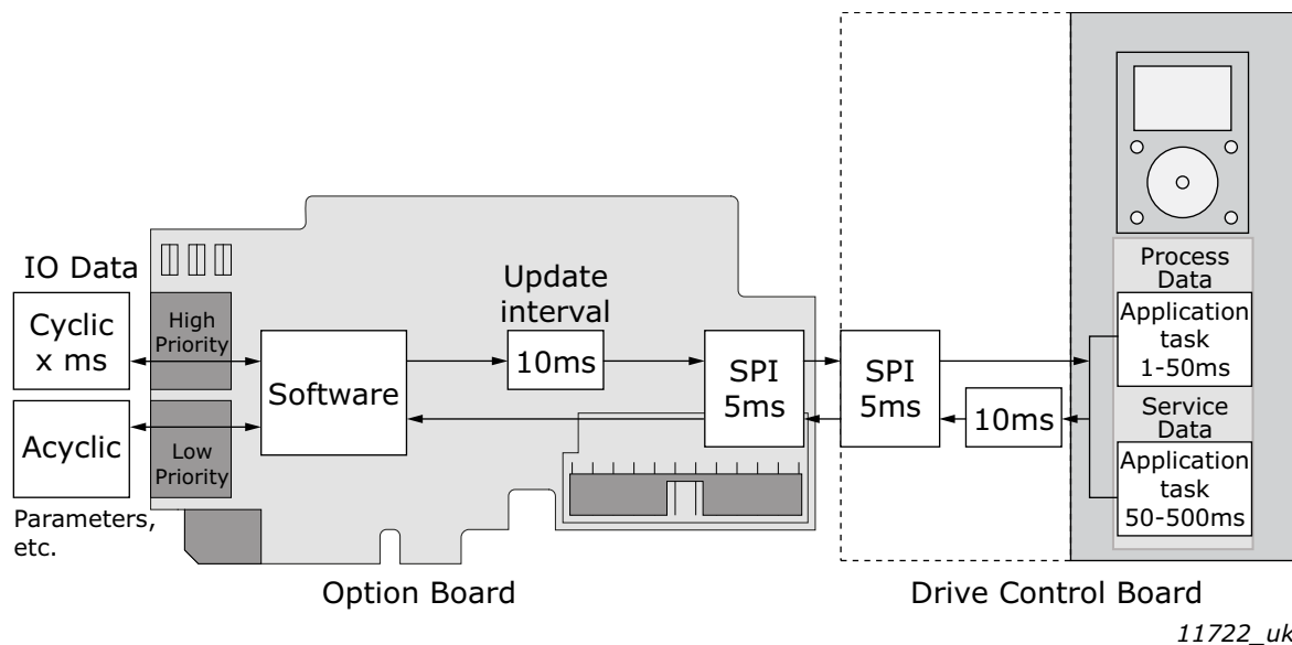
Figure 49. Normal fieldbus communication
