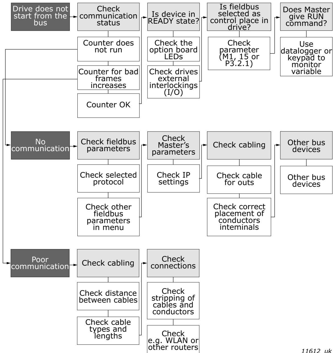
Figure 48. Fault tracing diagram for OPTE9
