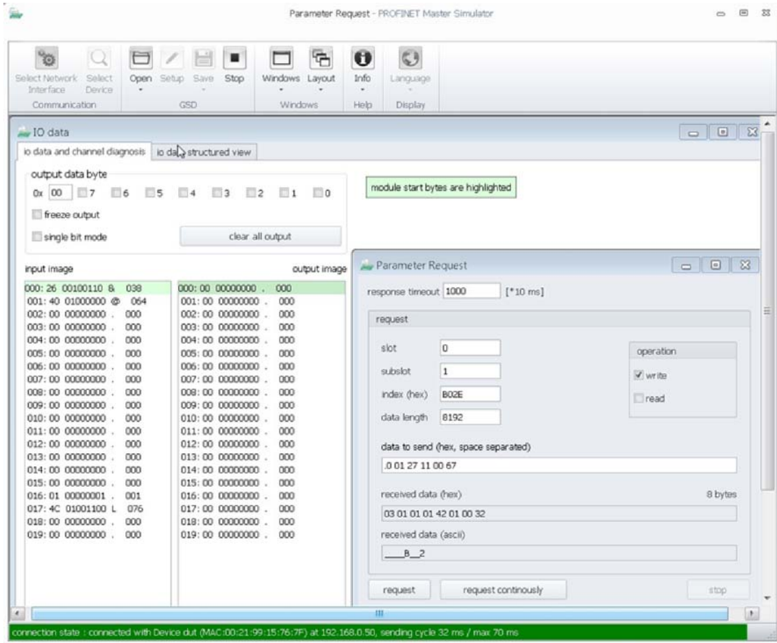
Figure 40. Screen capture from “PROFINET Master Simulator” requesting value for ID103.
