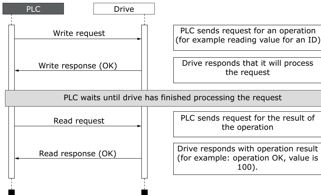
Figure 38. Successful parameter channel operation
