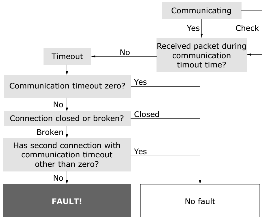
Figure 35. The Modbus TCP/UDP function in case of timeout
