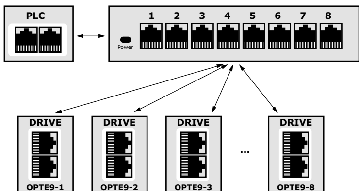
Figure 5. Star Topology
