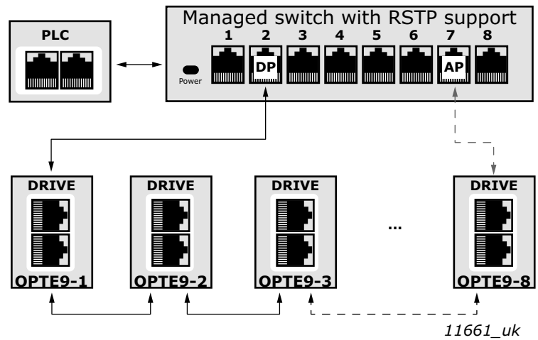
Figure 7. Ring topology
