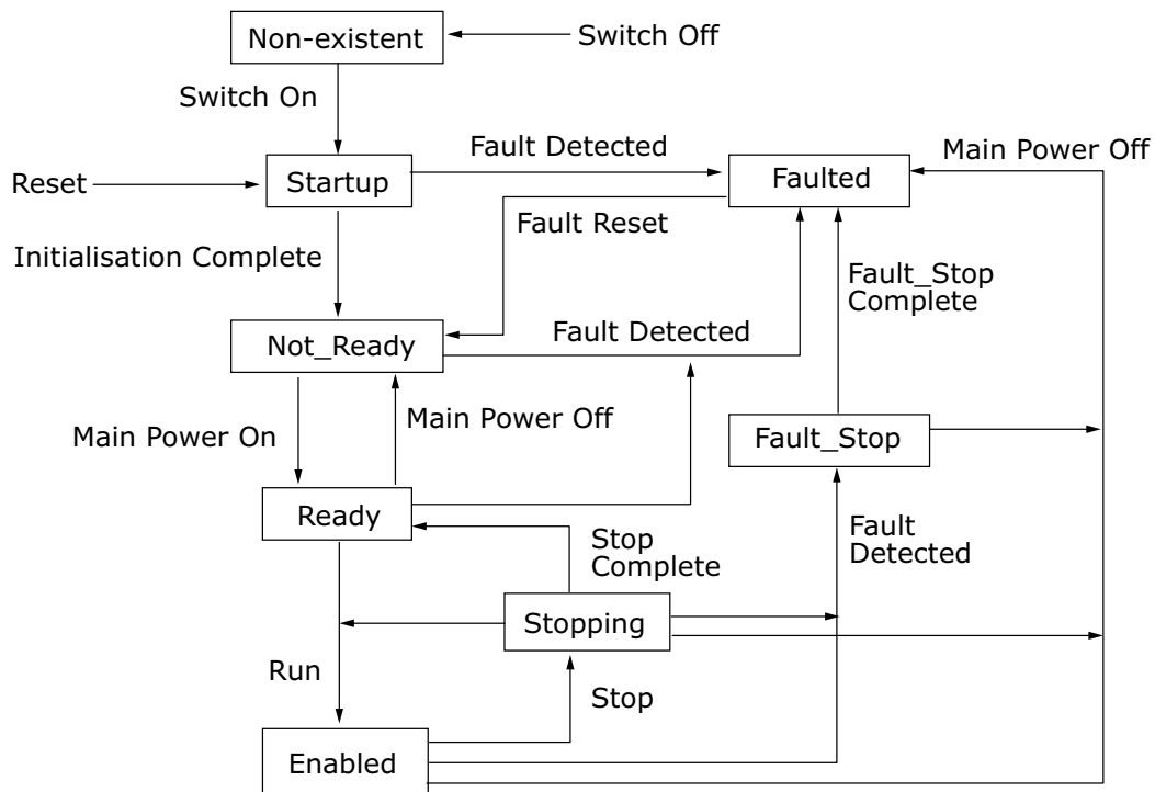
Figure 46. Control Supervisor State Machine
