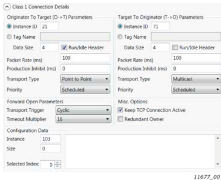
Figure 47. Configuration example from EIPScan Tool
