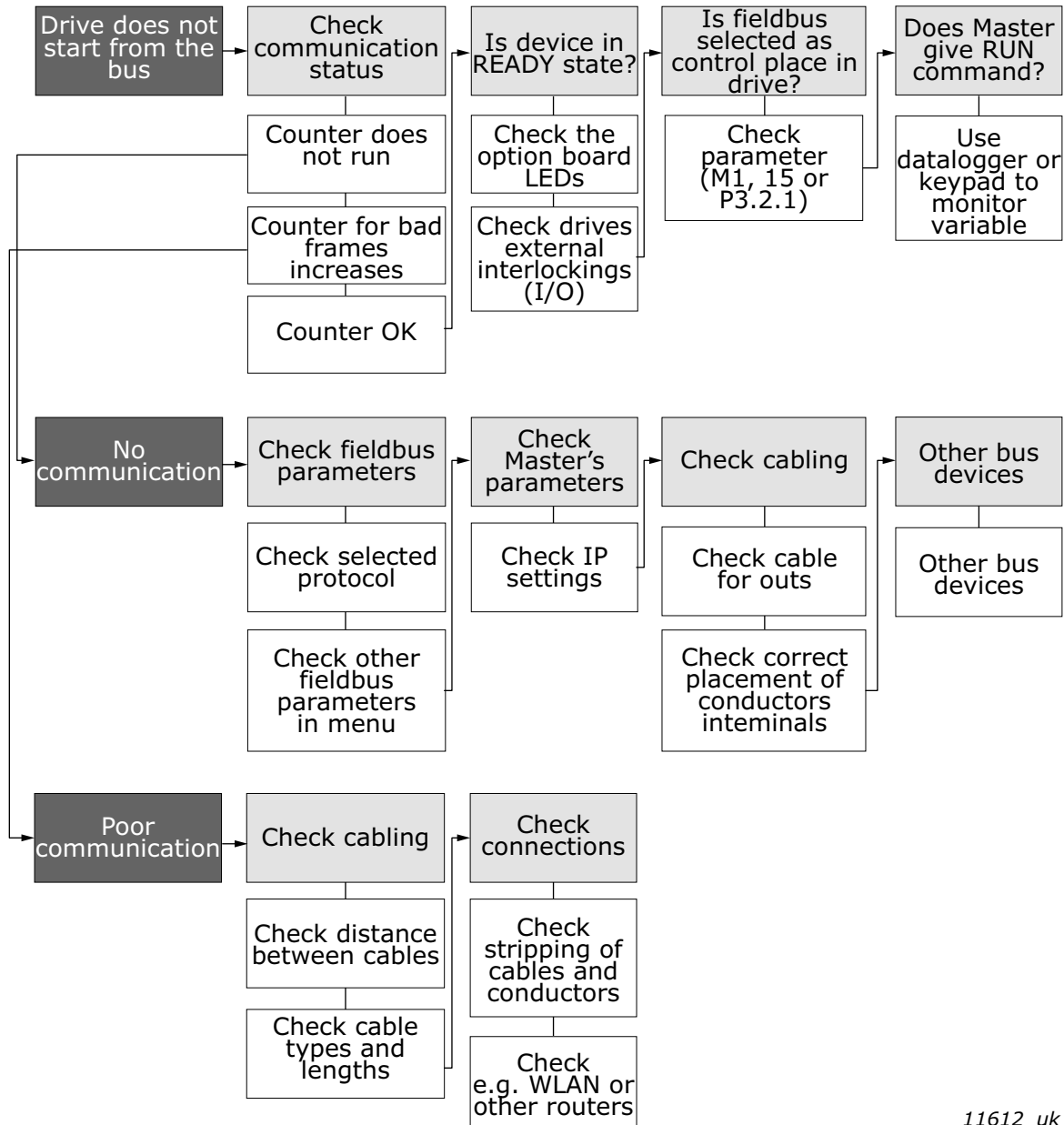
Figure 51. Fault tracing diagram for OPTE9
