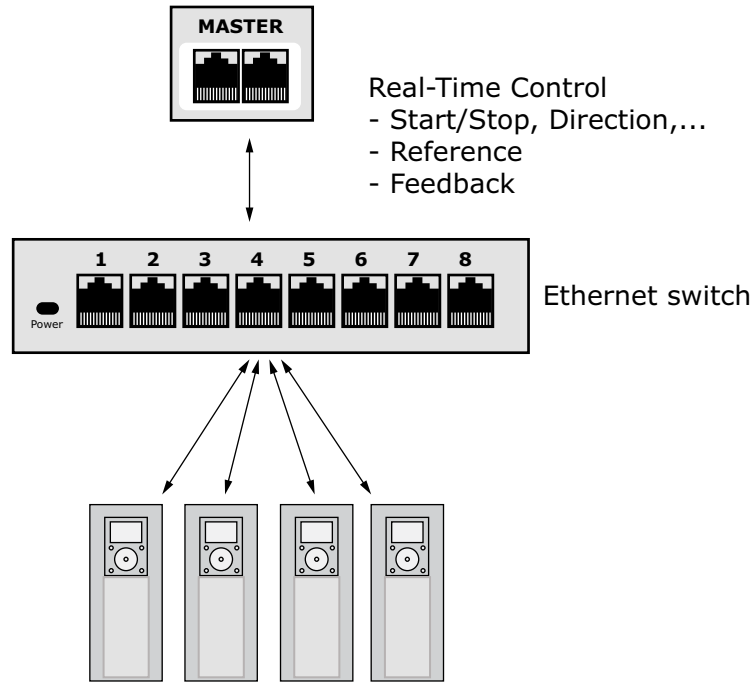
Figure 4. Ethernet, Machine to Machine
