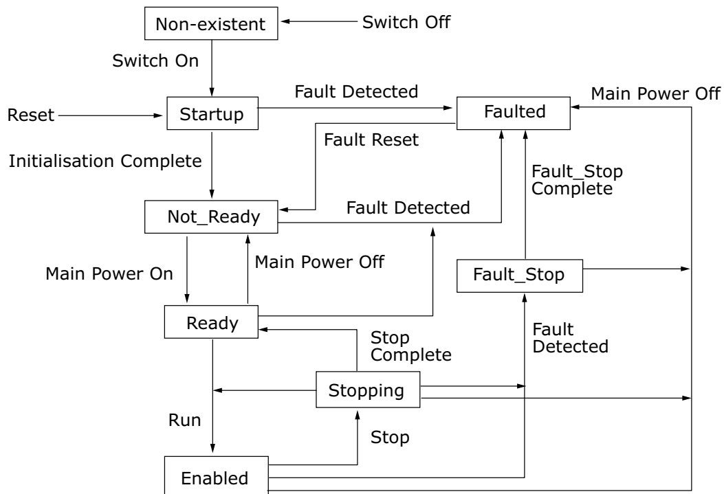
Figure 49. Control Supervisor State Machine
