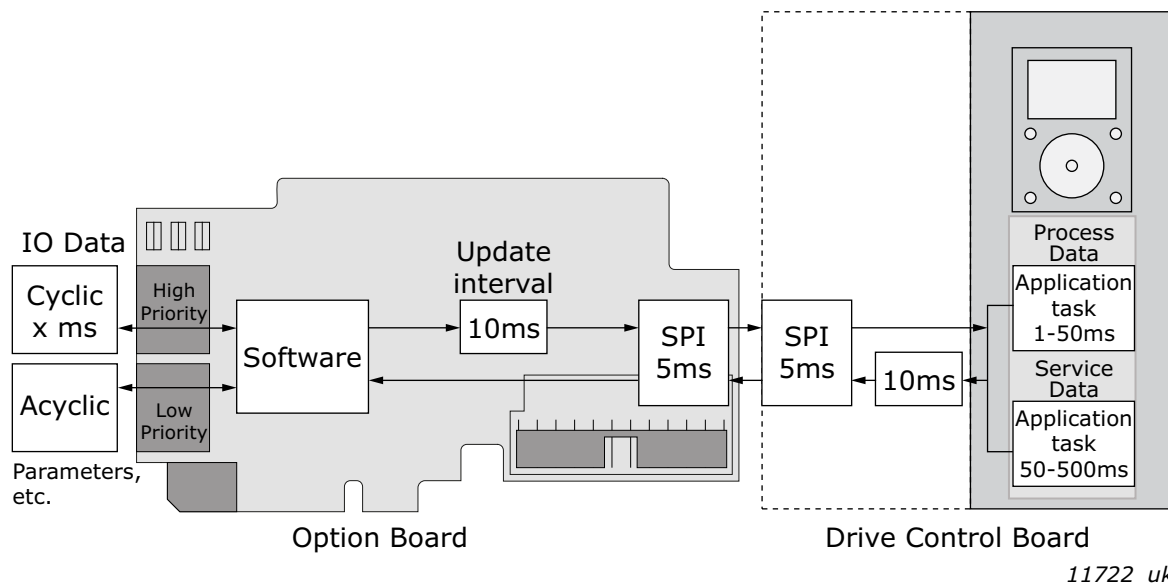
Figure 52. Normal fieldbus communication
