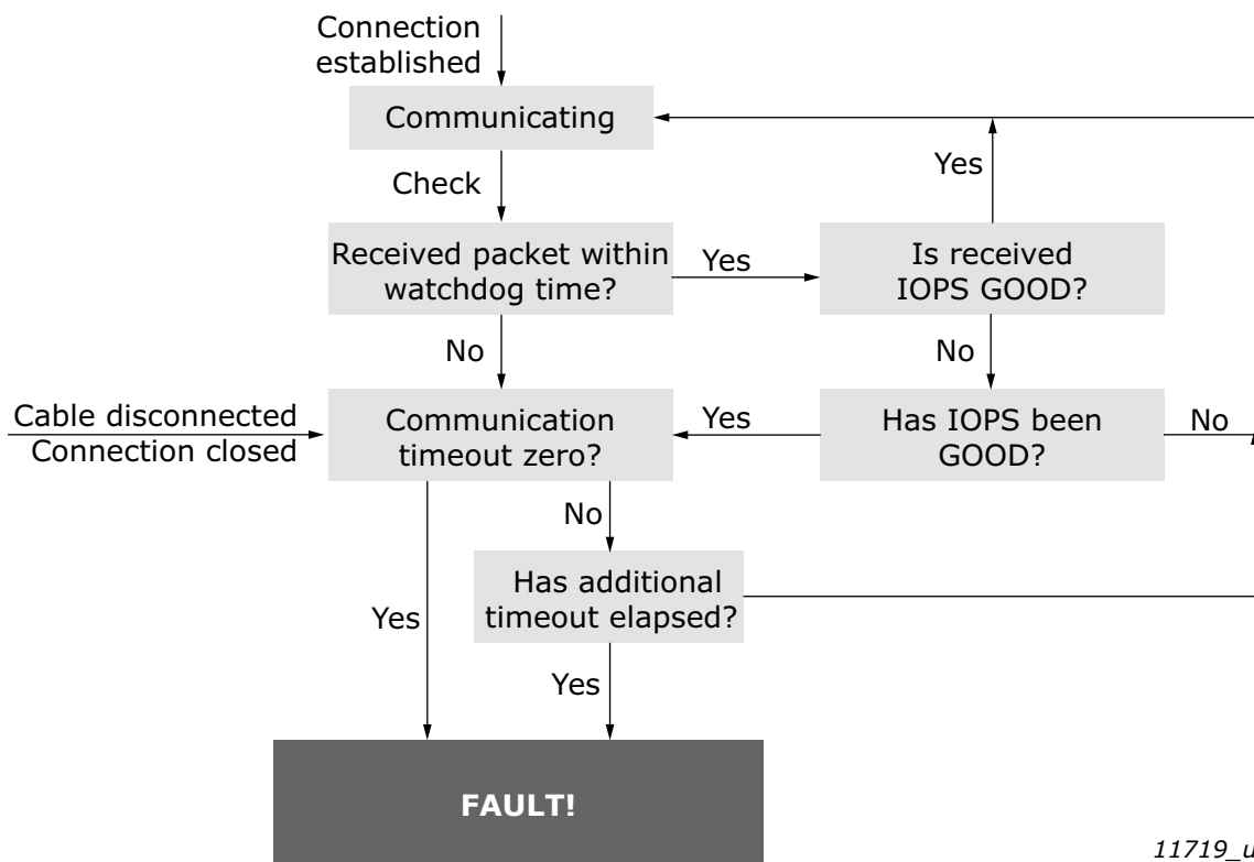
Figure 44. PROFINET IO communication and timeout fault
