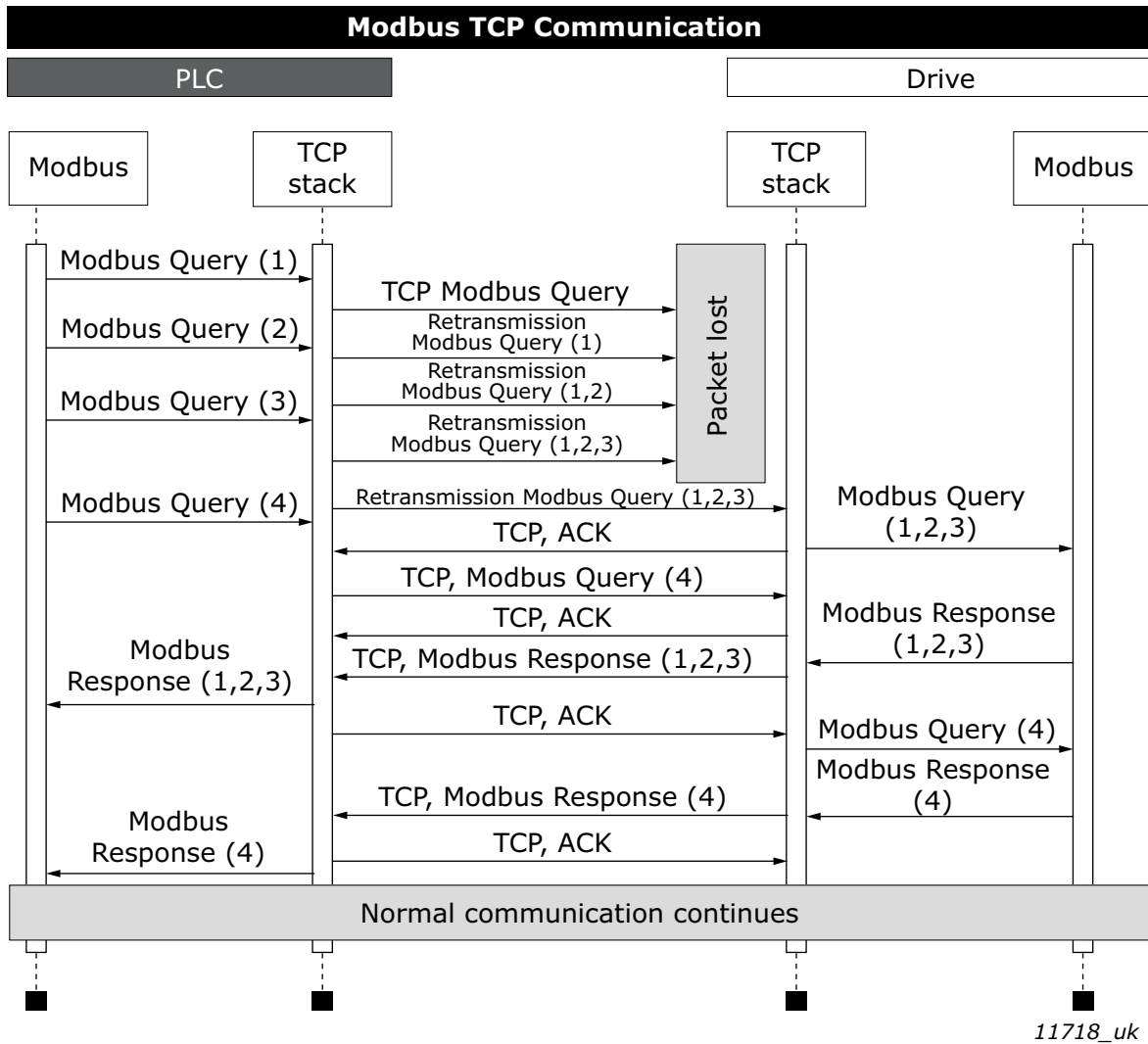
Figure 36. Modbus TCP retransmissions
