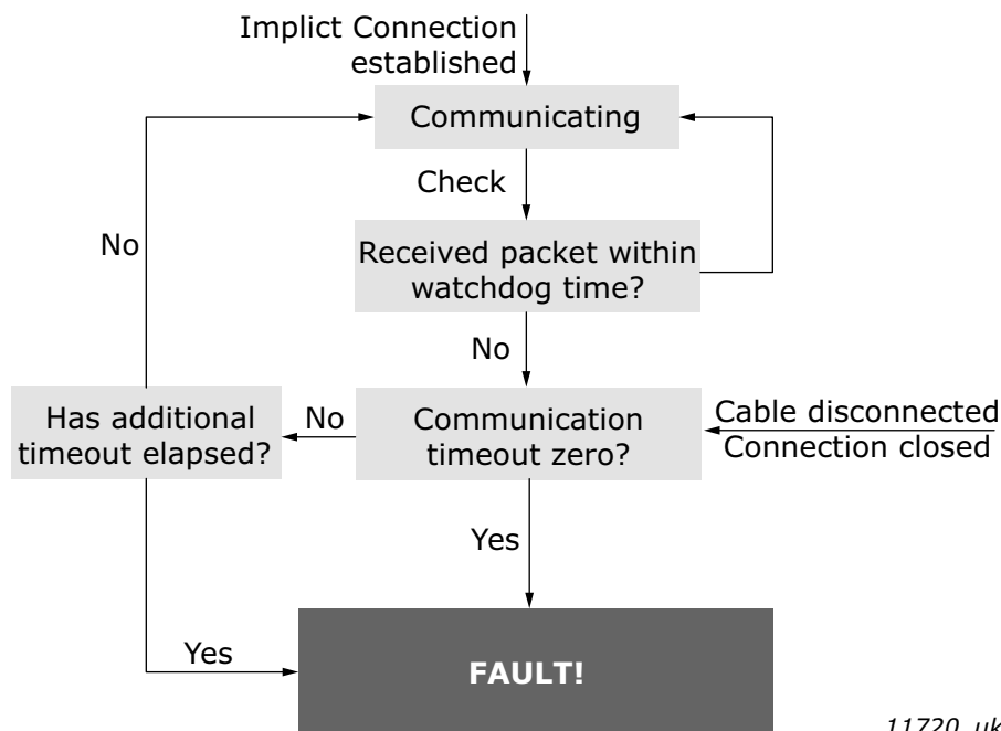
Figure 47. EtherNet/IP timeout logic with implicit connection (IO connection)
