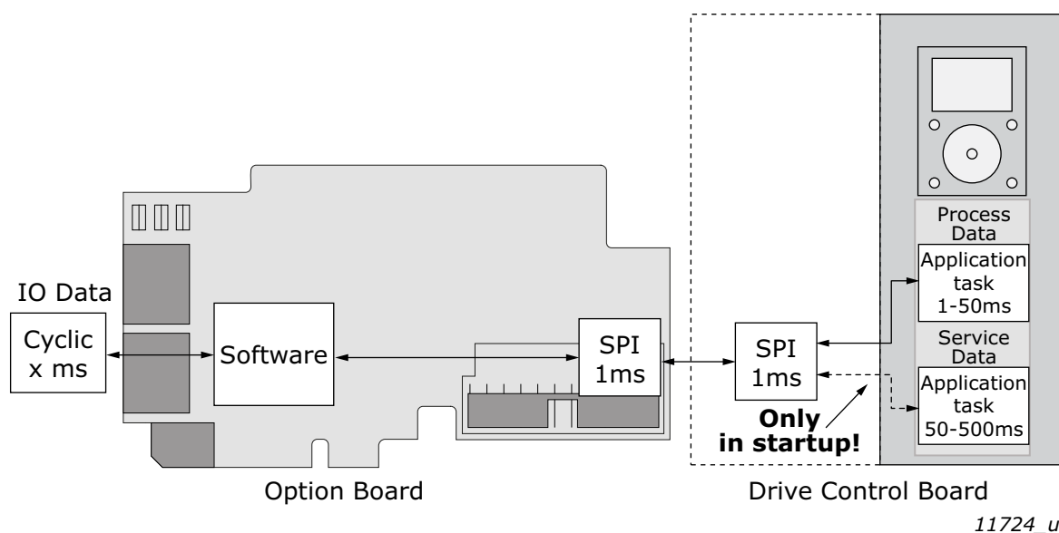
Figure 54. Fast PROFIBUS communication
