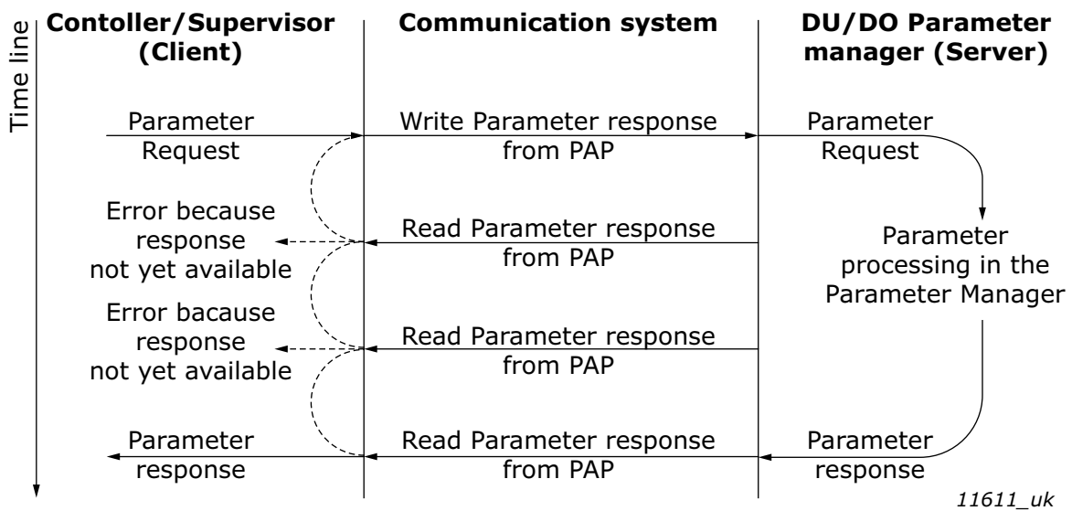
Figure 40. PROFINET parameter access model
