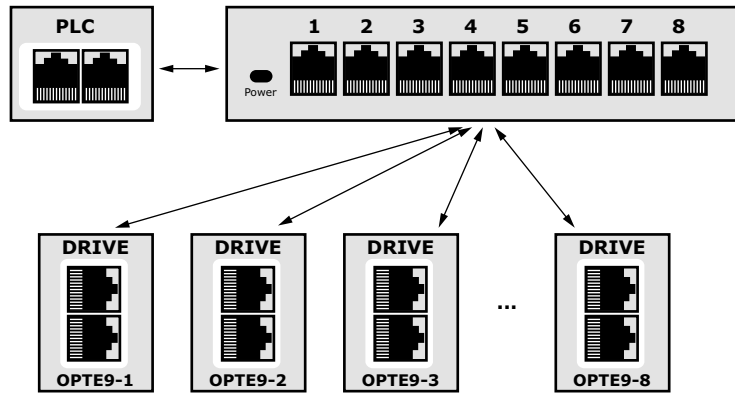
Figure 5. Star Topology
