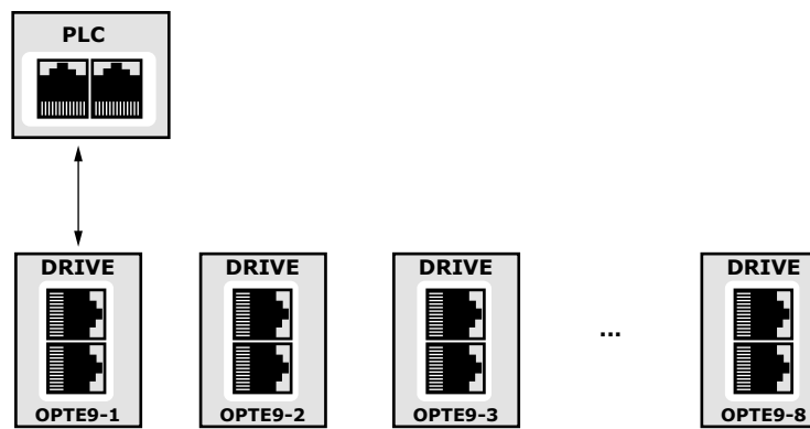
Figure 6. Daisy chain topology
