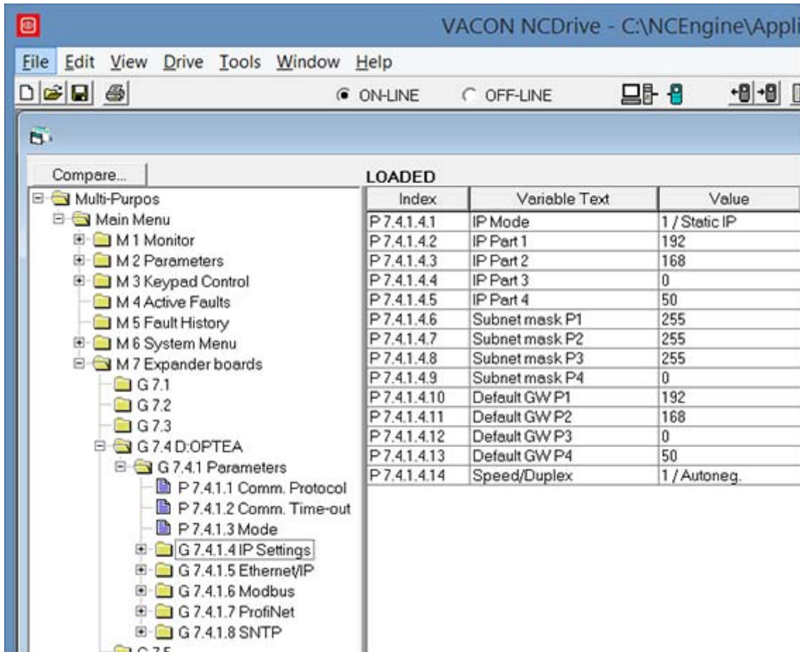
Figure 29. NC Drive: OPTEA parameters
