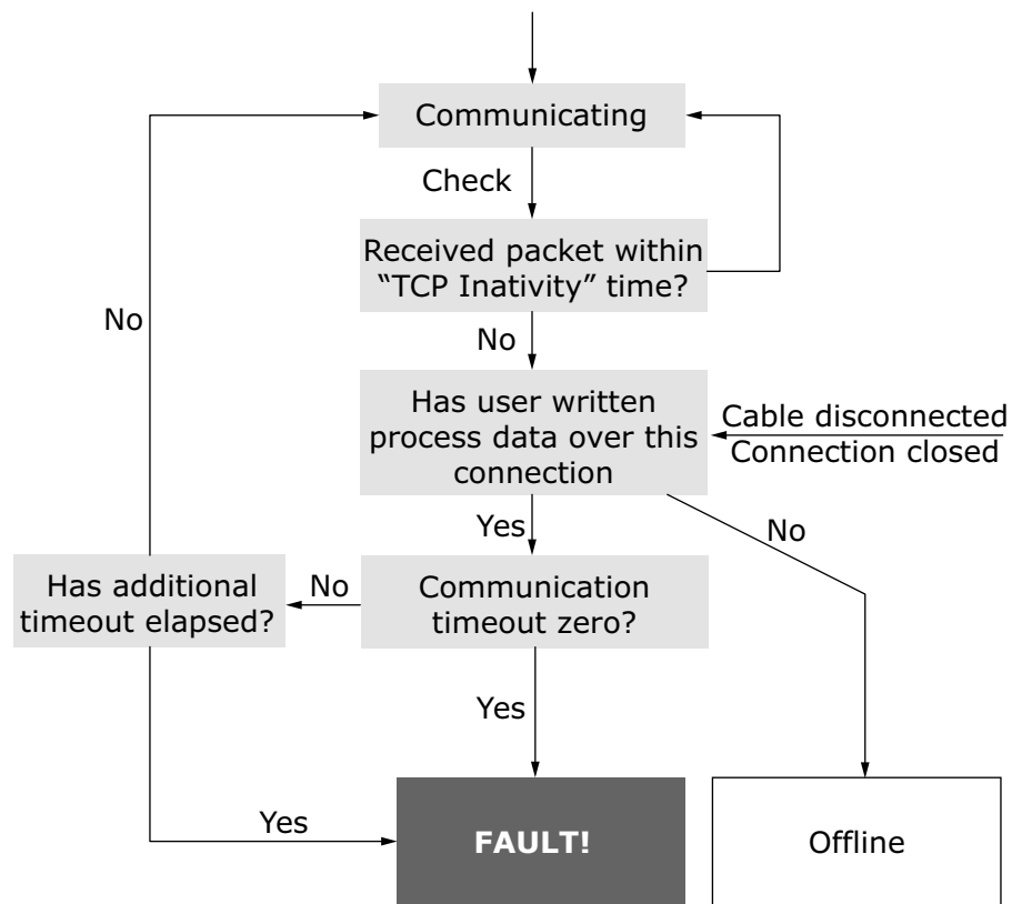
Figure 51. EtherNet/IP timeout logic with explicit connection
