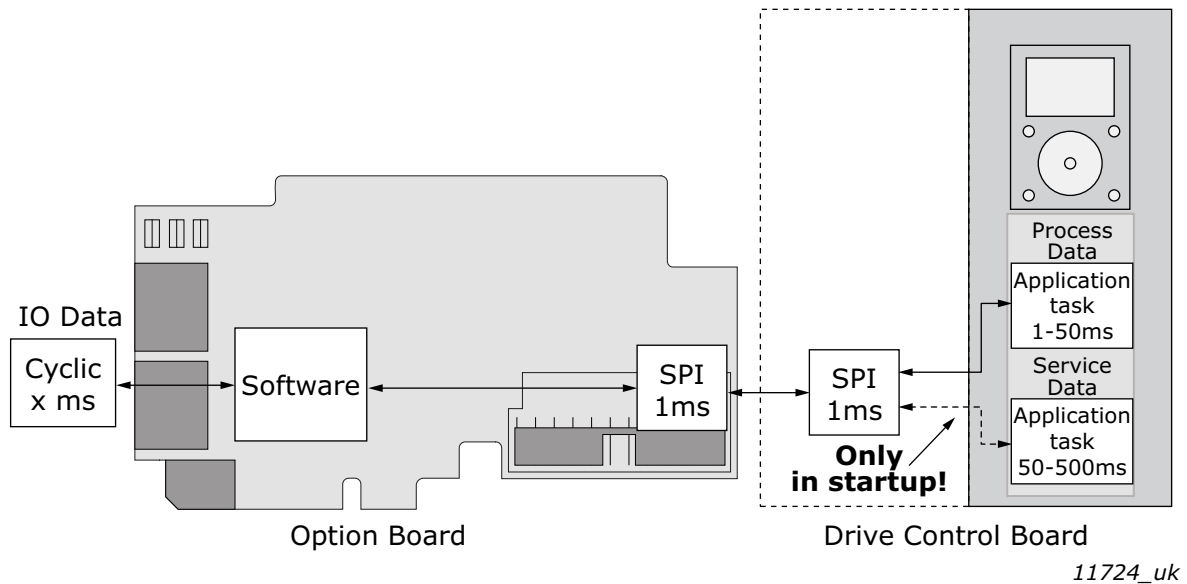
Figure 57. Fast PROFIBUS communication
